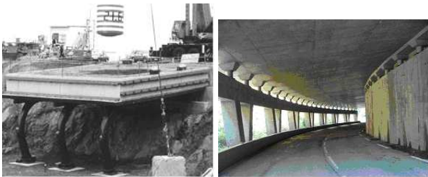
Fig. 12. Full-scale steel-concrete composite rock shed subjected to a falling weight (left; Maegawa et al., 2003), gallery with PSD dissipation system in Val d'Arly, France (right; taken from Masuya, 2007).
