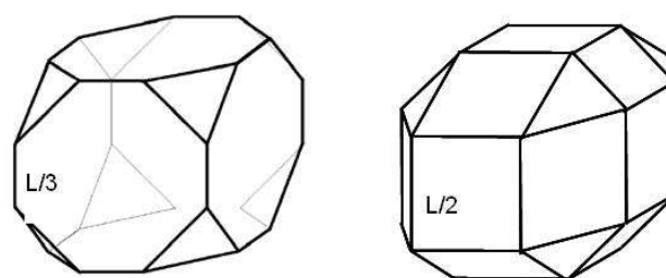
Fig. 21. Standardized test blocks for flexible rockfall protection systems related to a regular cube with edge length L according to the approval guidelines of Switzerland (left, Gerber, 2001a, until 2008) and the European Union (right, EOTA, 2008).
