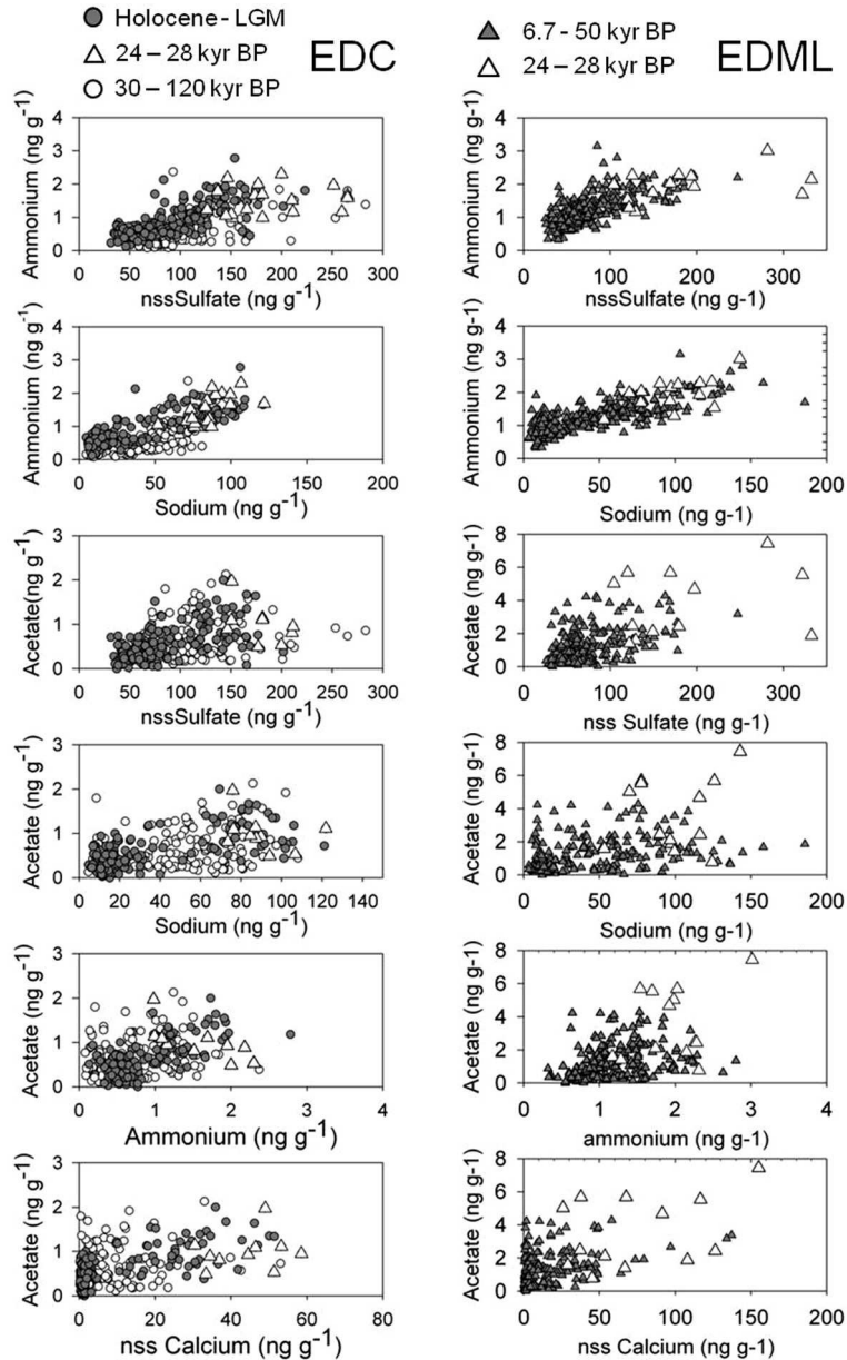
Fig. 4. Inter-species relationships (concentrations are expressed in \text{ng g}^{-1} ). From top to bottom: ammonium as a function of nss sulphate, ammonium as a function of sodium, acetate as a function of nss sulphate, acetate as a function of sodium, acetate as a function of ammonium and acetate as a function of nss calcium. EDC (left part): grey circles and white triangles correspond to the past 30 kyr (Holocene and LGM, samples reprocessed in 2001 and 2002), white triangles cover the 24–26.5 kyr BP time period (see text) and white circles correspond to the remaining part of the last climatic cycle (30–120 kyr BP, samples reprocessed in 2003 and 2006). EDML (right part): white triangles correspond to 24–28 kyr BP (see text) and grey triangles correspond to the remaining part of the past 50 kyr.
