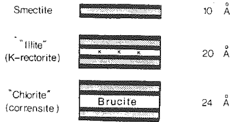
Schematic cross-sections of elementary clay particles. Smectite is represented as a single 2:1 silicate layer, "illite" as two 2:1 silicate layers coordinated by a single plane of K ions, and "chlorite" as two 2:1 silicate layers coordinated by a single brucite sheet. The dark bands represent the tetrahedral siloxane sheet and the stippled band the octahedral sheet (not to scale.)
