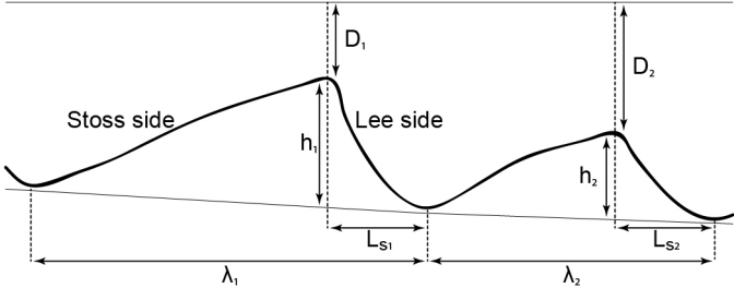
Figure 2 : Schematic representation of 1 and 2 dunes characteristics. \lambda is the wavelength, L_s is the lee side length, h is the height and D is the crest depth.
