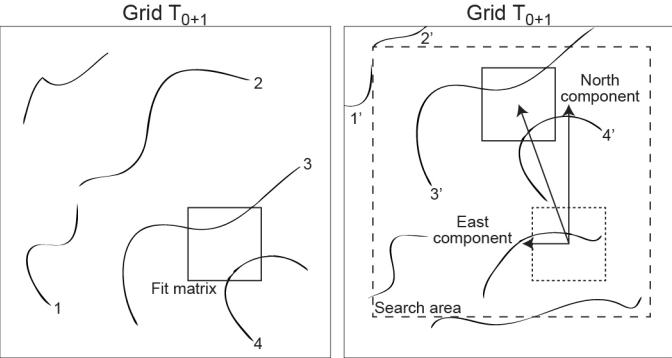
Figure 3 : Schematic representation of the cross-correlation technique to obtain the displacement field. For every grid point, a fit matrix for \text{DTM}_{t_1} defined at the moment t_1 is shifted in east and north directions within a search matrix for \text{DTM}_{t_2} defined at the moment t_2 . The search radius is defined from maximum assumed value of migration.
