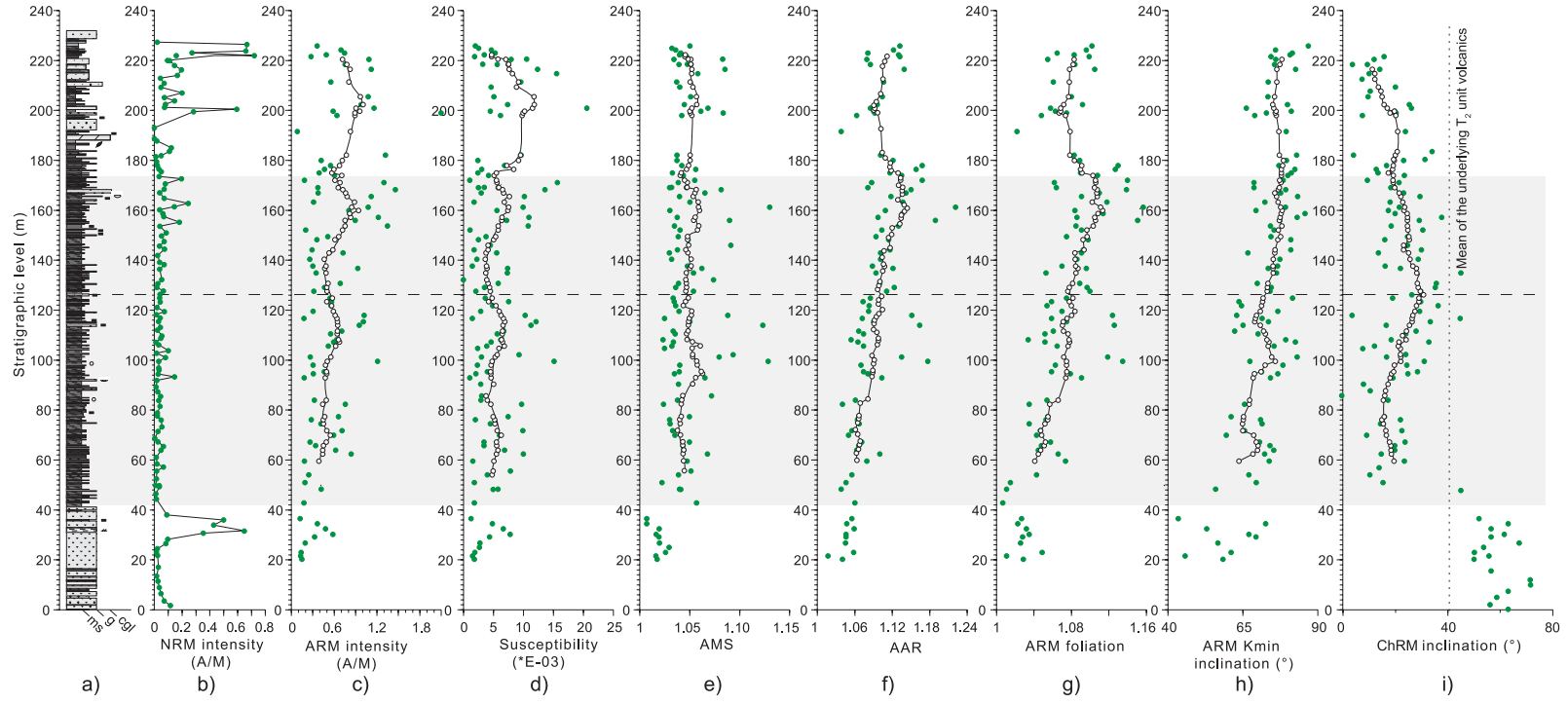
Figure 12. (a) Lithostratigraphy for the top of Unit T 2 and Unit T 3 . Natural remanent magnetization (NRM) intensity, Anhyseretic remanent magnetization (ARM) intensity (c), bulk susceptibility (d), anisotropy of magnetic susceptibility (AMS) (e), anisotropy of anhyseretic remanent magnetization (AARM) (f), foliation of anhyseretic remanent magnetization (ARM) (g), inclination of minimum ARM axis ( K_{\min} ) (h) and ChRM inclination (i) plotted against depth (0 is bottom; 240 m is top). Dots are the measured values; circles linked by short line are the mean values of every ten adjacent measured values. Note that the anomalously high ChRM inclinations of the tuff layers from the top of Unit T 2 probably reflects secular variation as interpreted by Dupont-Nivet et al. (2010b).
