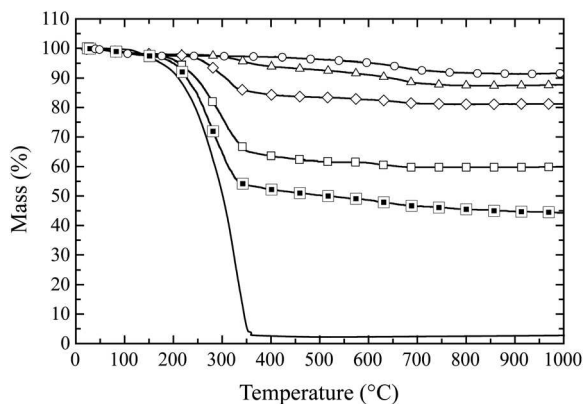
Fig. 7 Thermograms of Na-Mt (white circles), C_{10}E_3 -Mt hybrid organoclay (triangles for a lateral monolayer arrangement of C_{10}E_3 , lozenge as a lateral bilayer organization, squares for a normal bilayer and black squares for a normal tilted bilayer arrangement respectively) and bulk C_{10}E_3 (solid line).
