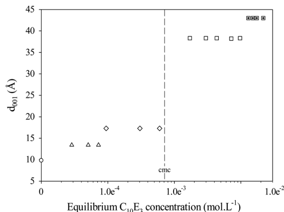
Fig. 5 Evolution of the d_{001} basal spacing determined by the 001 reflection of the silicate sheets obtained from SAXS profiles of Mt in white circles, and \text{C}_{10}\text{E}_3 -Mt hybrid organoclays (triangles for a lateral monolayer arrangement of \text{C}_{10}\text{E}_3 , lozenge as a lateral bilayer organization, squares for a normal bilayer and black squares for a normal tilted bilayer arrangement respectively) as a function of the equilibrium \text{C}_{10}\text{E}_3 concentration.
