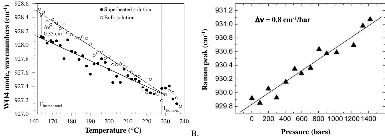
Fig. 5: A. Spectroscopic pressure measured by the Raman shifts of the tungstate dissolved in tensile solutions trapped in SFI. B. Calibration at positive pressure.
