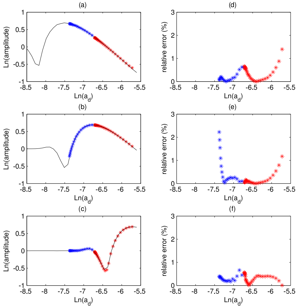
Figure 6. (a–c) Ridge functions extracted from the source-corrected WR_e of homogeneous layers of thicknesses \Delta z = 22, 45 and 130 cm, respectively: for the HR (red: a_d \in \mathcal{R}_{a_d}^{HR} ) and VHR (blue: a_d \in \mathcal{R}_{a_d}^{VHR} ) sources of the seismic SYSIF device. The solid black line stands for the reference ridge function performed with a_d \in \mathbb{R}^+ . (d–f) Associated relative errors between the source-corrected and reference ridge functions.
