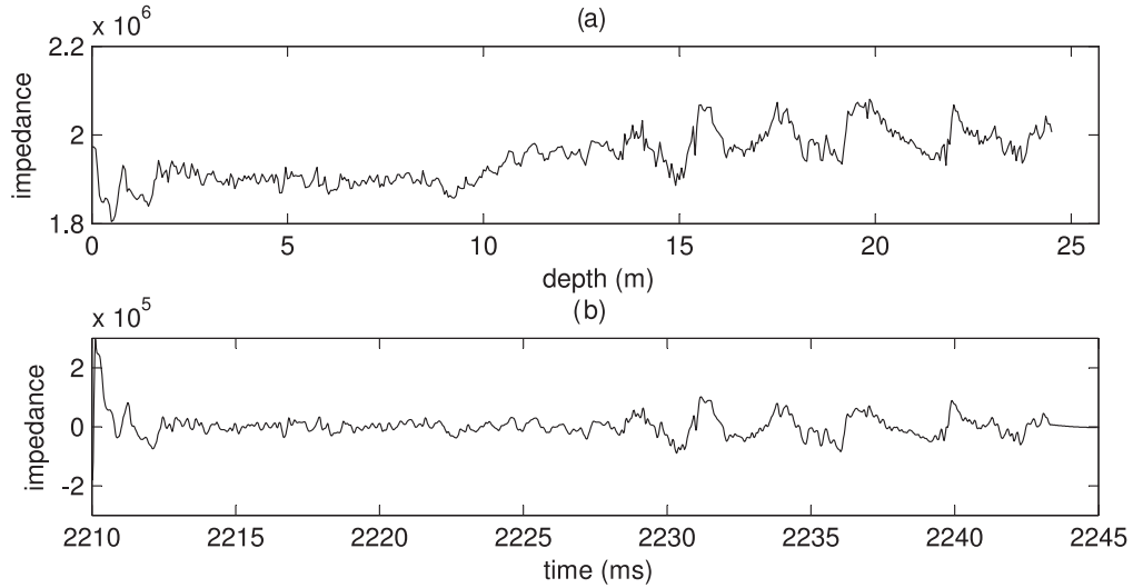
Figure 8. (a) Acoustic impedance profile (unit: \text{Pa}\cdot\text{s}\cdot\text{m}^{-1} ) obtained from density and sound velocity measurements on ground truth data as a function of depth. (b) Relative acoustic impedance profile reconstructed with the inverse wavelet transform of the reference WR ( a \in \mathbb{R}^+ ) as a function of the two way traveltime.
