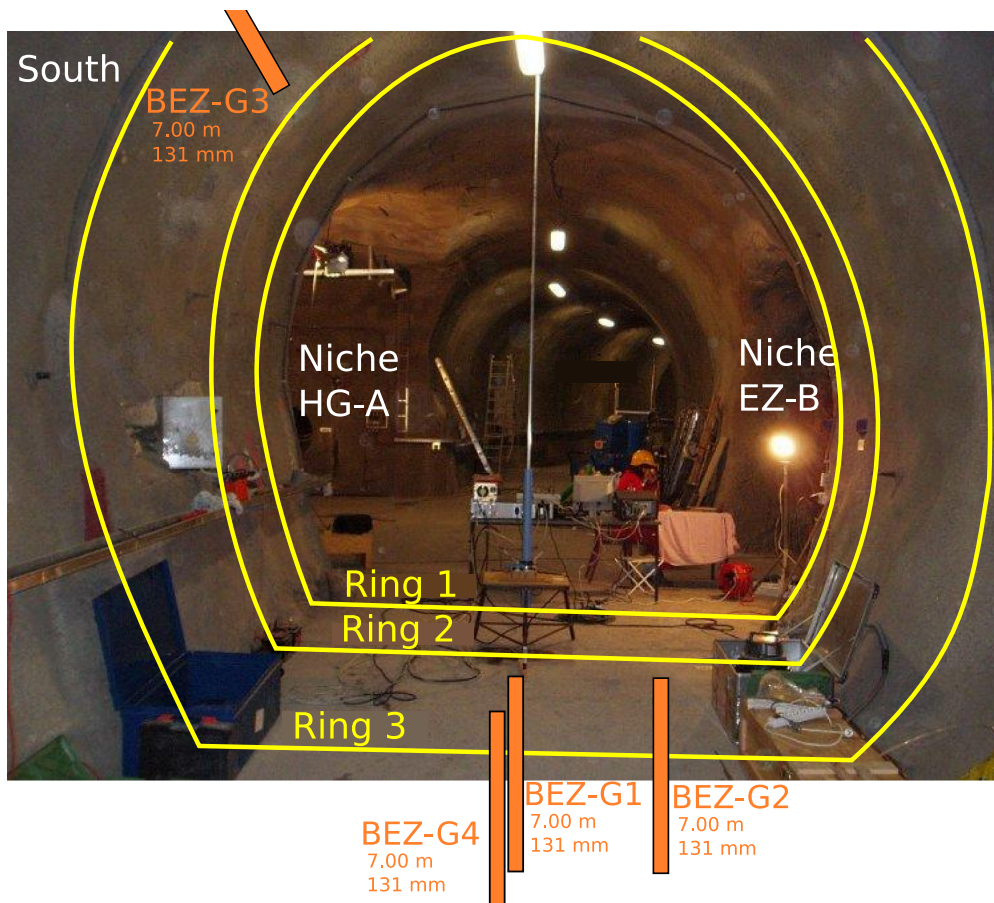
Figure 6. Picture at the entrance of gallery 04 and scheme of the electrodes rings and boreholes equipped for electrical measurements.
