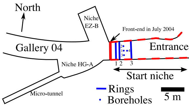
Figure 3. Top view of the gallery 04 entrance including the rings and boreholes location. The red line indicates the position of the gallery front-end in 2004 July and the start niche is represented by the red dashed line. Boreholes BEZ-G1, G2 and G4 are vertical downwards, while BEZ-G3 is oblique upwards (see Fig. 6).
