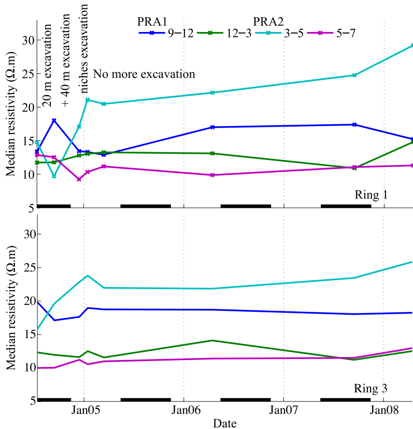
Figure 11. Evolution of the median resistivity with time in the different sectors surrounding the gallery from the surface to a depth of 1.5 m. Black lines indicate summers as the gallery environment is more humid in summer than in winter. Graphics correspond to rings 1 and 3 from top to bottom. The location of the different sectors are represented Fig. 8 with the corresponding colours.
