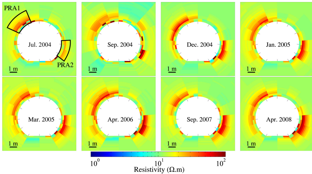
Figure 7. Evolution of the average resistivity with time during the process of gallery 04 excavation from 2004 July to 2008 April. North is on the right side.
