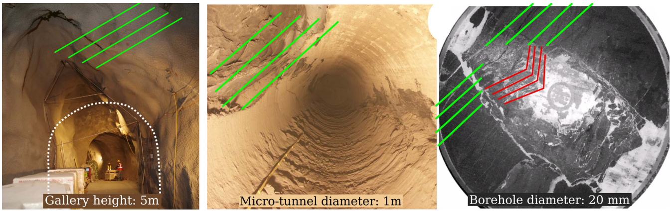
Figure 2. Influence of the bedding on buckling observed at different scales. From left to right: around the EZ-A niche of the Mont Terri laboratory (photo: Comet photoshopping, Zürich), around the HG-A microtunnel and around a borehole (photos: Mont Terri project, Swisstopo). The bedding is represented by the green lines.
