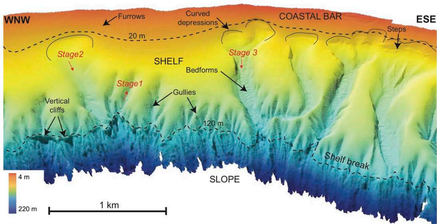
Figure 7. 3D view of the canyon heads of the Etang-Salé area (vertical exaggeration x3), isobaths at 20 m and 120 m are indicated. The interpretation of the different stages of canyon formation is indicated in red.
