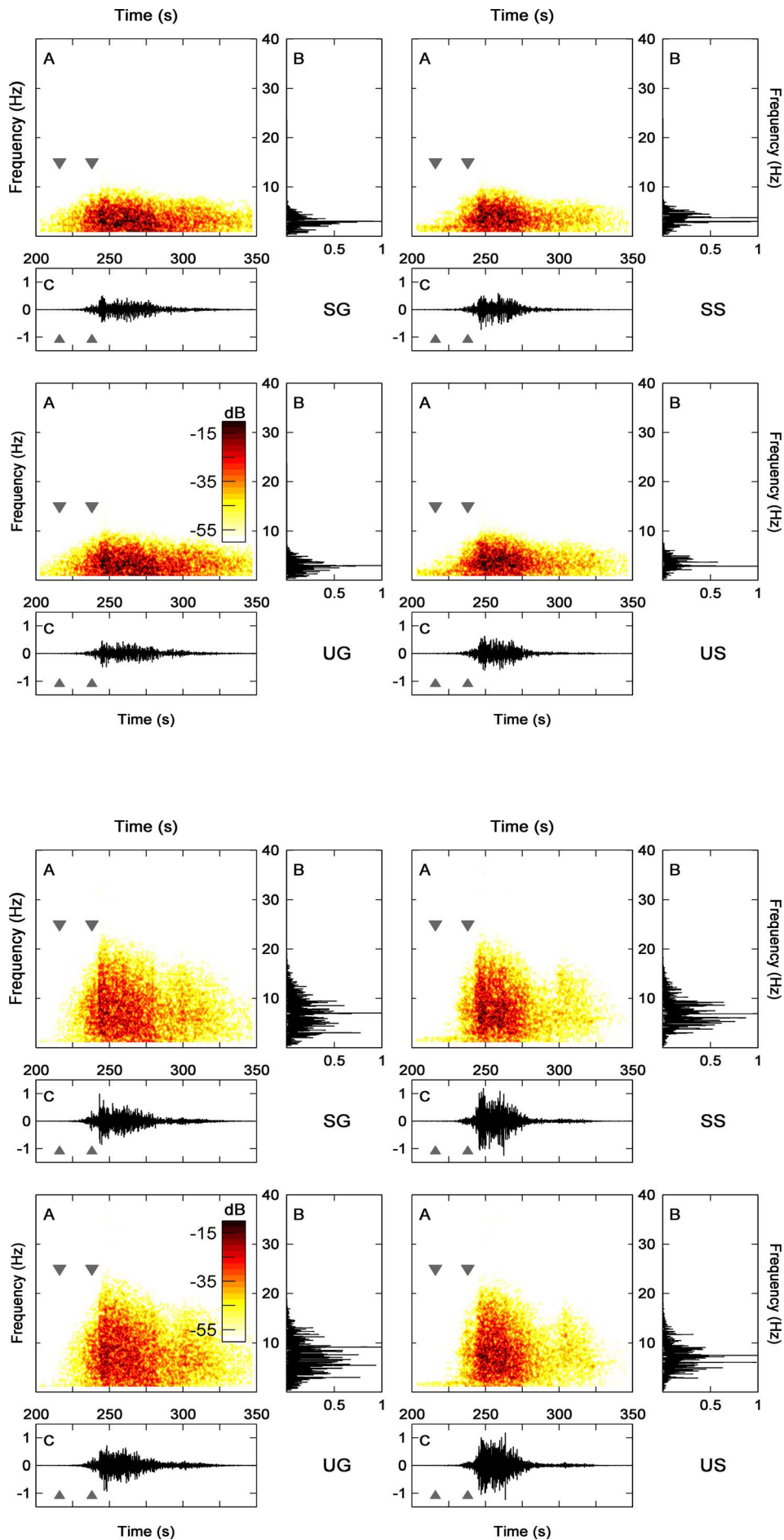
FIG. 6. (Color online) Simulated T-phase arrivals at hydrophone M7 (347 km), generated by a 4 Hz Gaussian seismic source. Each group of spectrogram (A), normalized spectrum (B), and time signal (C) corresponds to a combination (SG, SS, UG, US) of velocity profiles (see Table I). Data are shown with the same representation as Fig. 2. Arrows refer to T-wave arrival times in the actual data at M7 (Fig. 2).
