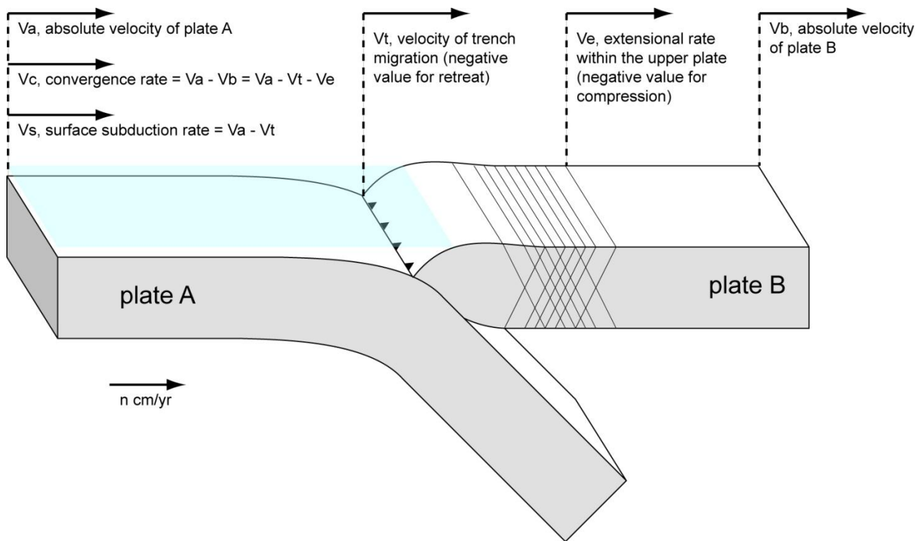
Figure 3 – Definition of convergence and subduction rates ( V_c and V_s respectively), considering absolute plate motions ( V_a and V_b ), absolute trench velocity ( V_t ) and extensional rate within the upper plate ( V_e ). For the sake of clarity, velocities are here considered horizontal and perpendicular to the trench, but oblique convergence is included in the kinematic reconstructions. Directions and lengths of arrows are arbitrarily chosen.
