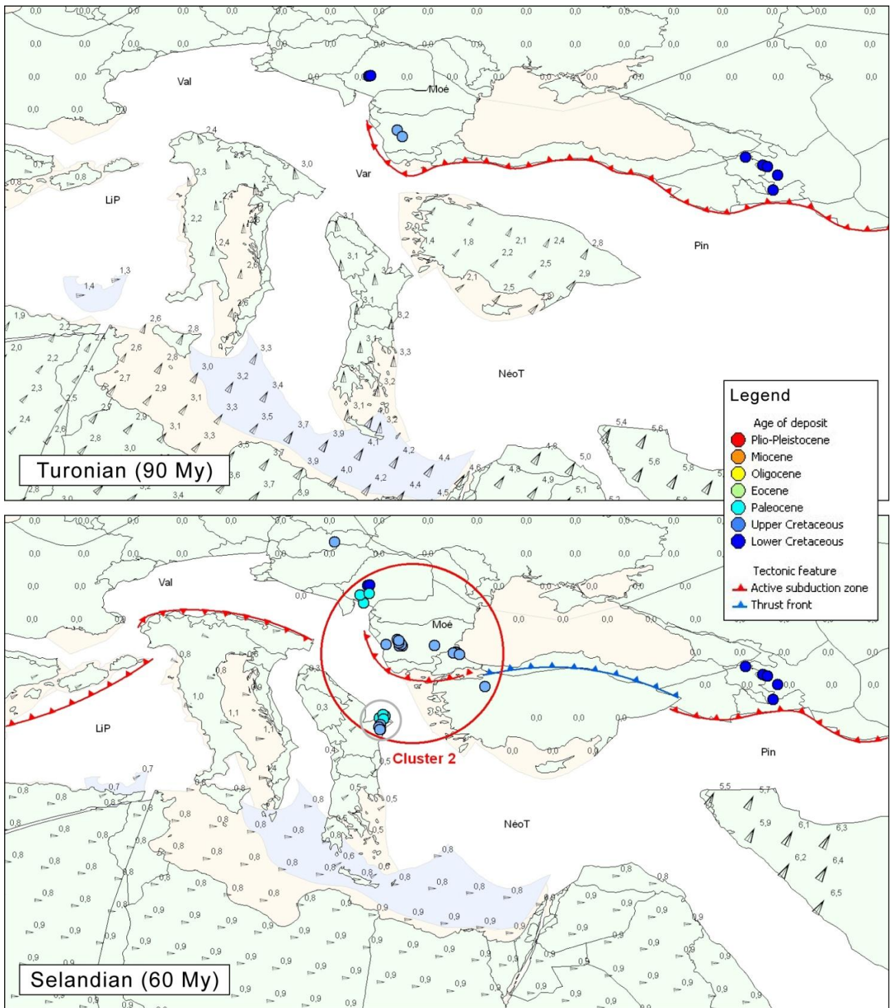
Figure 5a – Paleotectonic reconstructions and instantaneous velocity field of the western Tethys region in Turonian (top) and Selandian (bottom), using the UTIG PLATES global kinematic model (see Appendix 1). Eurasia is considered stable (fixed plate). Appearance of deposits in the subducting plate (small light grey circle) is a bias due to inaccurate plate boundary definition in the original plate tectonic model. Val: Valaisan ocean; LiP: Liguro-Piemontese ocean; Moë: Moesian platform; Var: Vardar ocean; Pin: Pindos ocean; NeoT: Neotethys ocean.
