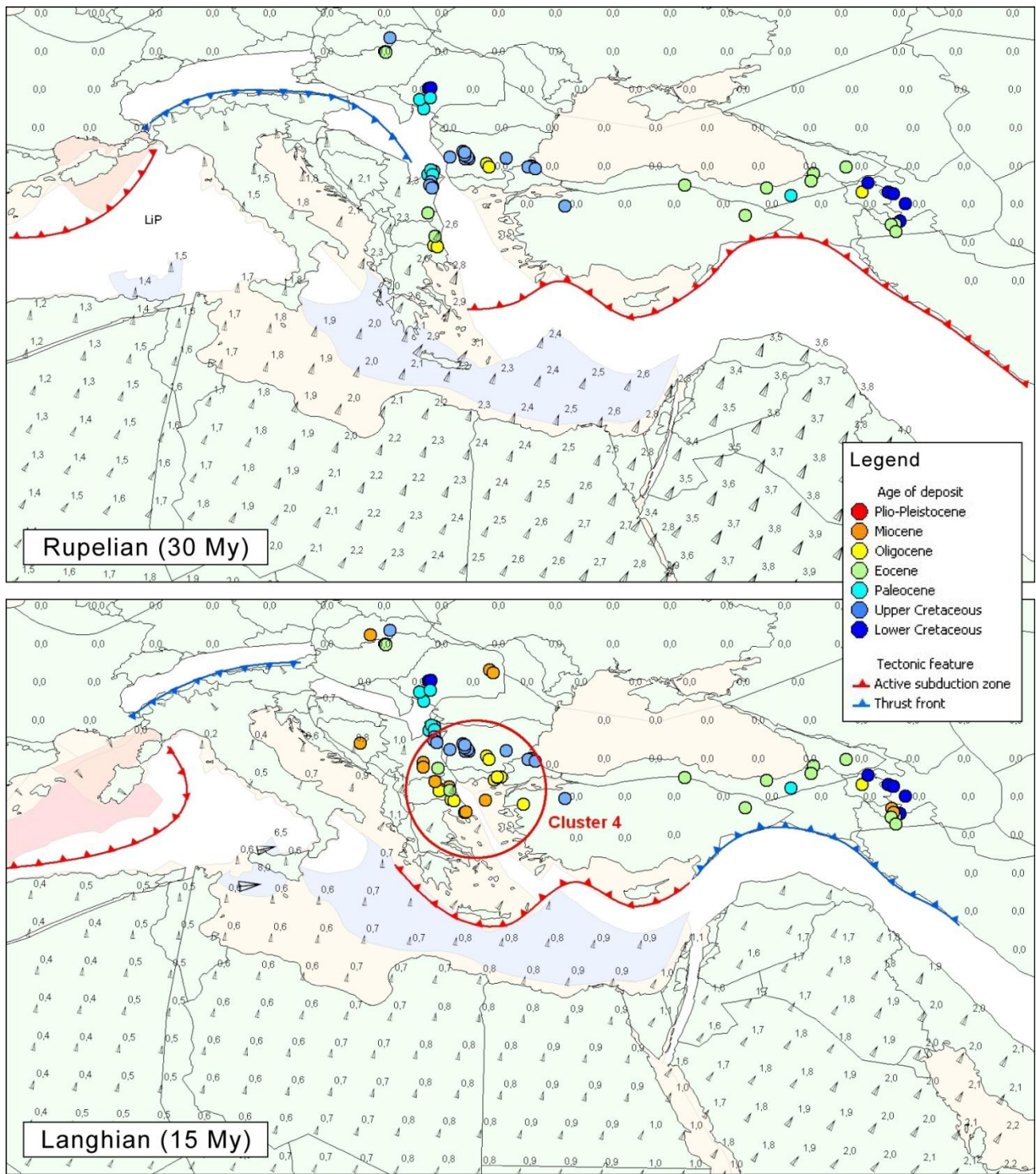
Figure 5b – Paleotectonic reconstructions and instantaneous velocity field of the western Tethys region in Rupelian (top) and Langhian (bottom), using the UTIG PLATES global kinematic model. Eurasia is considered stable (fixed plate). LiP: Liguro-Piemontese ocean.
