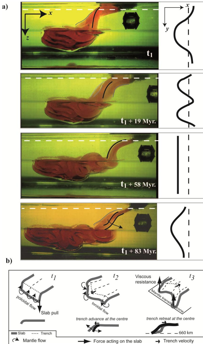
Figure 2 – a) Laboratory experiment number 13 from Guillou-Frottier et al. (1995), where lateral undulations (perpendicular to pictures) are underlined by black (front) and grey (back) lines, and illustrated by thick black lines at the right of each picture corresponding to horizontal cross-sections (at the level of dashed white lines); b) From left to right, temporal evolution of the 3D shape during the buckling behavior (lateral and vertical folding) of a subducting lithosphere, with implications for trench retreat or advance.
