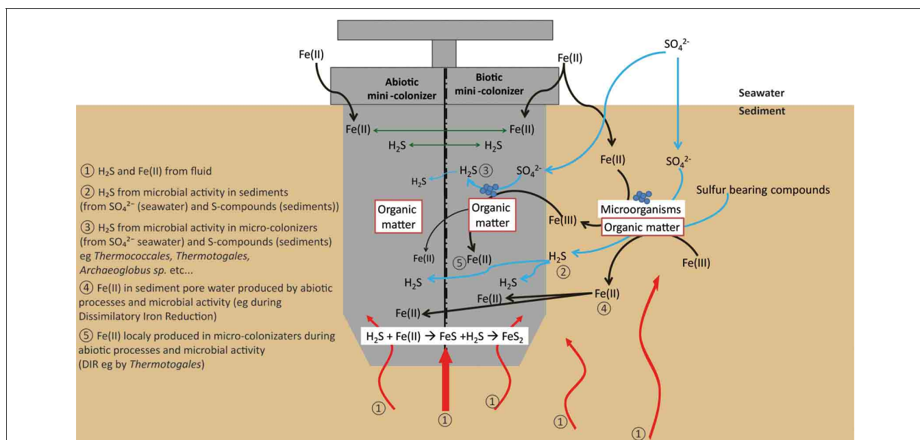
FIGURE 10 | Schematic diagram showing the different pathways for pyrite formation in both biotic and abiotic mini-colonizers.
