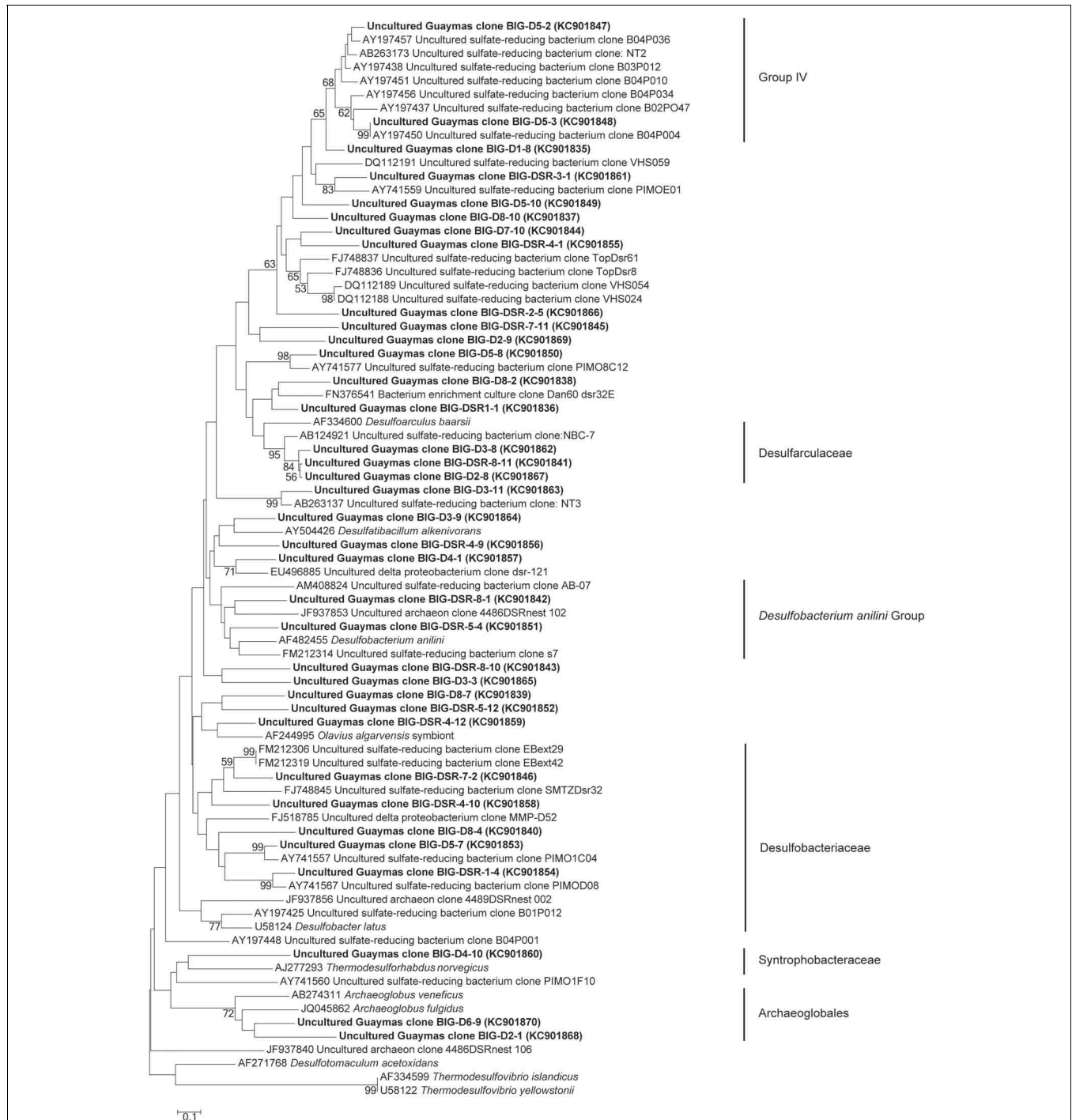
FIGURE 6 | Neighbor-joining phylogenetic tree of predicted amino acid translations of partial dsrAB gene. Bootstrap values above 50% based on 1000 replicates are reported.
