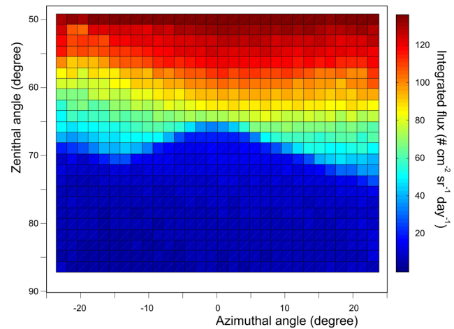
Figure 9. Observed integrated muon flux, after an acquisition time of about 30 days.
