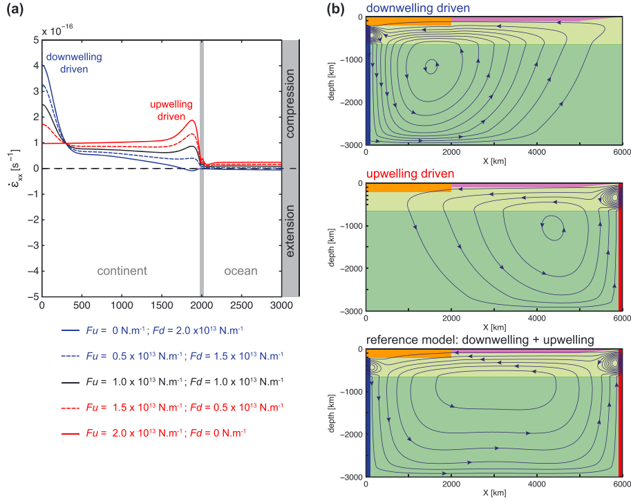
Figure 6. (a) Strain rate at the surface across the 3000 km long continental and oceanic lithospheres ( L=0 km and l_c=2000 km, see Figure 3a). (b) Streamlines obtained for the downwelling driven model ( F_u=0 \text{ N m}^{-1} , F_d=2 \cdot 10^{13} \text{ N m}^{-1} ), the upwelling driven model ( F_u=2 \cdot 10^{13} \text{ N m}^{-1} , F_d=0 \text{ N m}^{-1} ), and the reference model ( F_u=10^{13} \text{ N m}^{-1} , F_d=10^{13} \text{ N m}^{-1} ).
