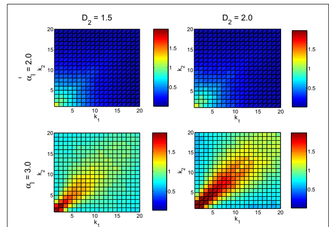
FIGURE 6 | The degree correlation matrix C(k_1, k_2) for different DFN model parameters \alpha_l and D_2 . This figure should be compared with Figure 5.
