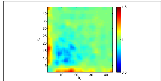
FIGURE 5 | Plot of the correlation matrix C(k_1, k_2) based on the equivalent networks generated from the eighth outcrop fracture data sets.
