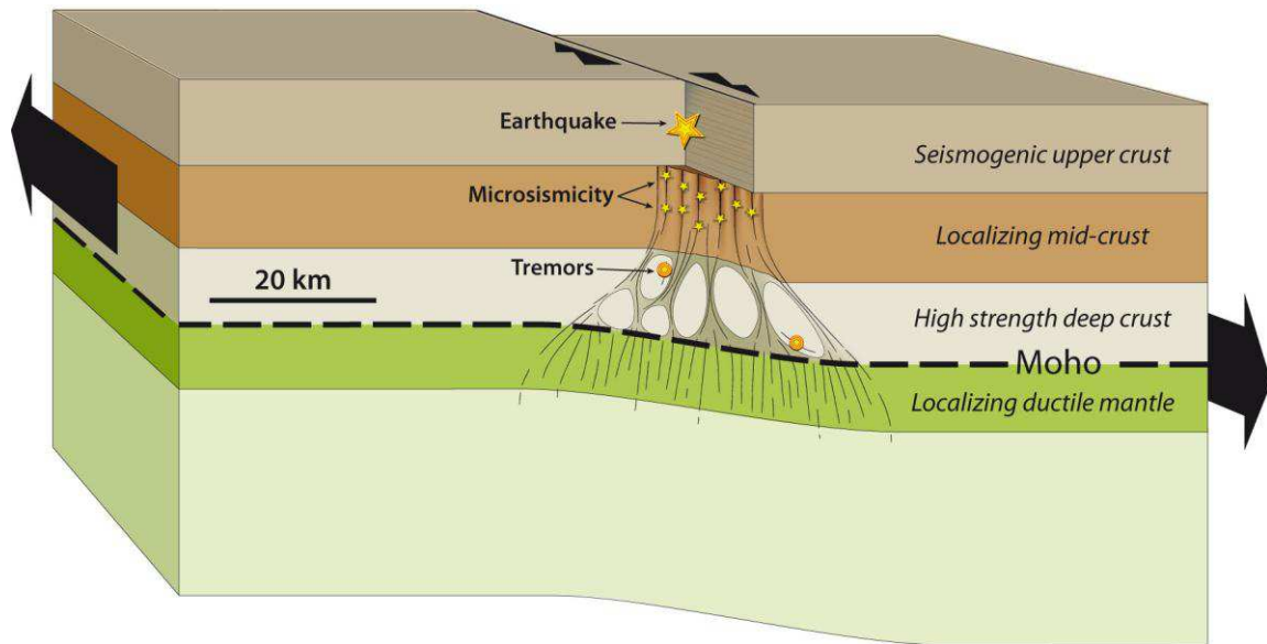
Figure 6: Schematic diagram of the mechanical layer of a continental strike-slip plate boundary showing, from top to bottom: the seismogenic upper crust; a weak, ductile mid-crust where deformation localizes into ductile shear zones as the fraction of layered rock increases; a strong, ductile, lower crust where deformation does not localize spontaneously but where shear failure is possible due to transient loading and pore pressure increase; a weak upper mantle where grain size reduction localises deformation into a ~50 km wide ductile shear zone.
