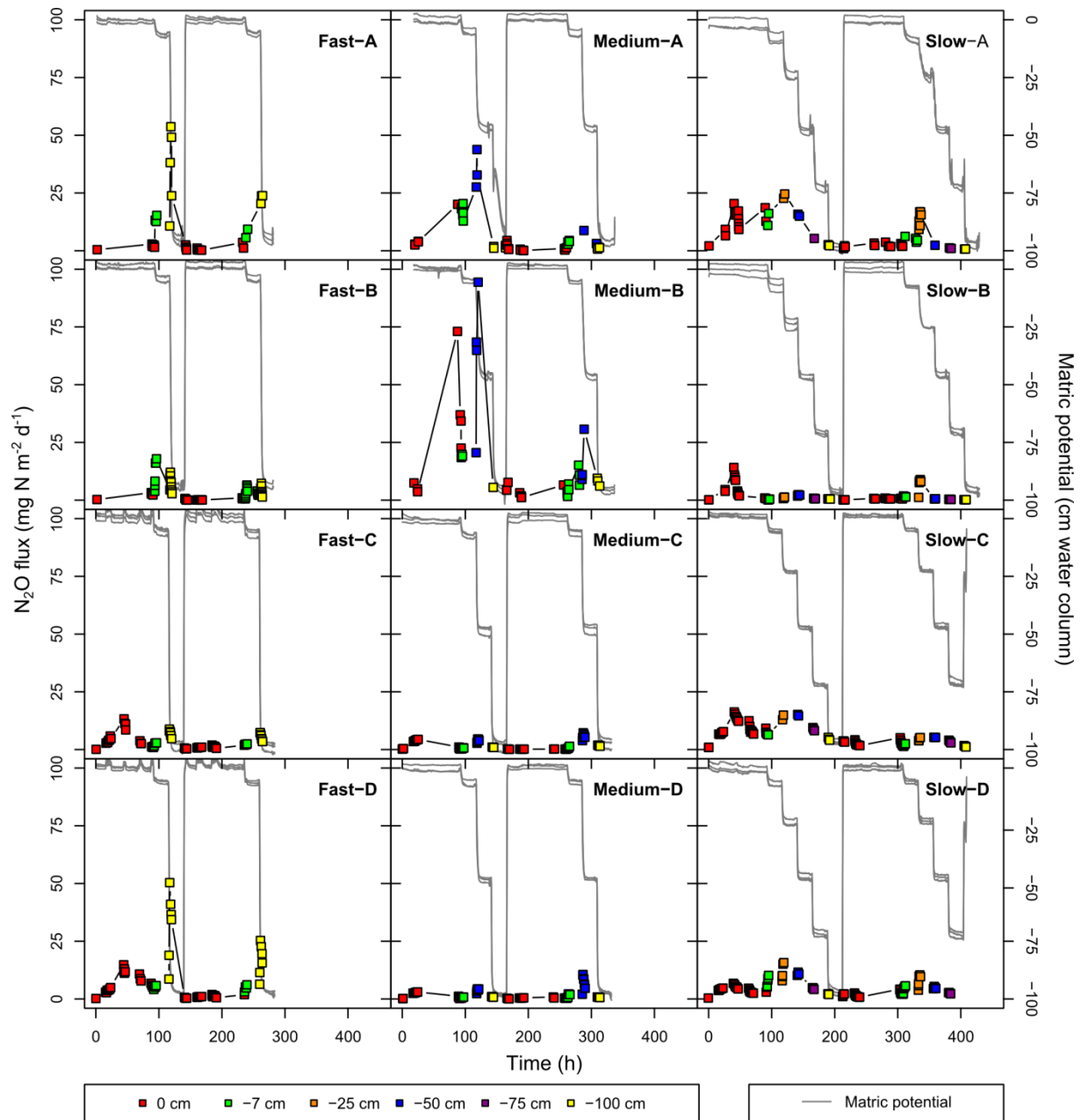
Fig. 2. Monitoring of the N 2 O fluxes of the 12 soil samples and the soil matric potential by the three tensiometers (Fast: 3 values of decreasing pressure head, Medium: 4 values, Slow: 6 values). For the sake of readability, the measurement points are linearly interpolated.
