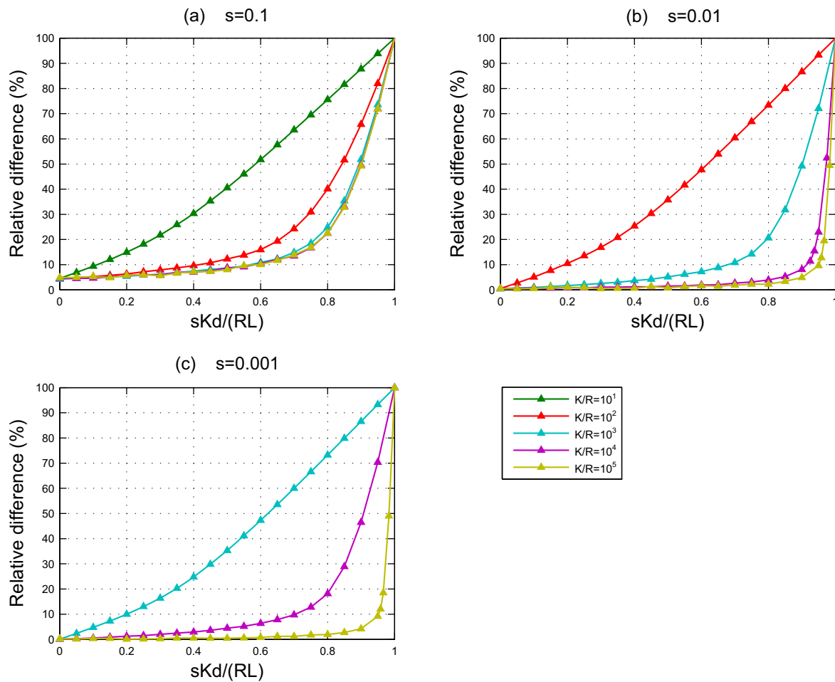
Figure 5. Relative difference between the full-depth and the Dupuit solutions, defined by (\{L_s\}_{full-depth} - \{L_s\}_{Dupuit}) / \{L_s\}_{full-depth} \times 100 , as a function of the ratio sKd/(RL) . Results for different values of K/R and (a) s = 0.1 , (b) s = 0.01 , and (c) s = 0.001 .
