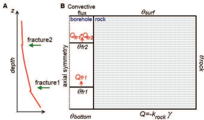
Figure 3: Illustration of the flow and temperature propagation simulation in a borehole. Borehole temperature profile with inferred fracture positions (A) and corresponding heat transfer model boundary conditions (B). We consider the heat diffusion and advection of heat with a constant vertical laminar flow in the borehole and the heat diffusion in the surrounding rock matrix. For each borehole section we impose the borehole flow as the sum of all fractures inflows and outflows ( Q_{fr} ) below the modeled section (shown by red).
