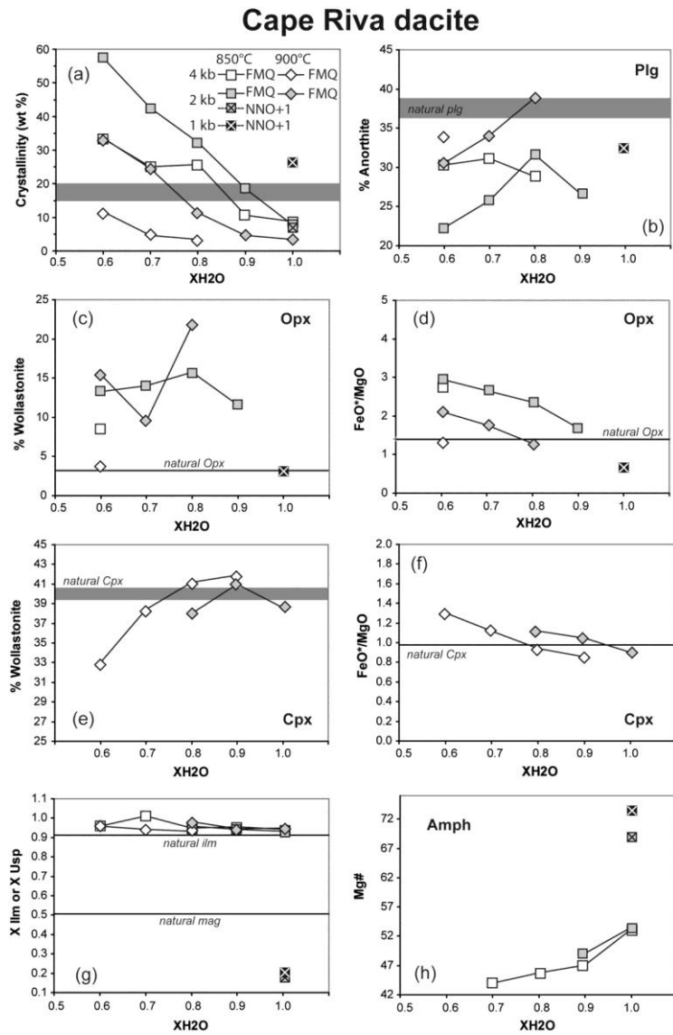
Figure 12. Crystallinity and mineral compositions of the Cape Riva dacite as a function of XH 2 O. Same legend as Figure 11.
