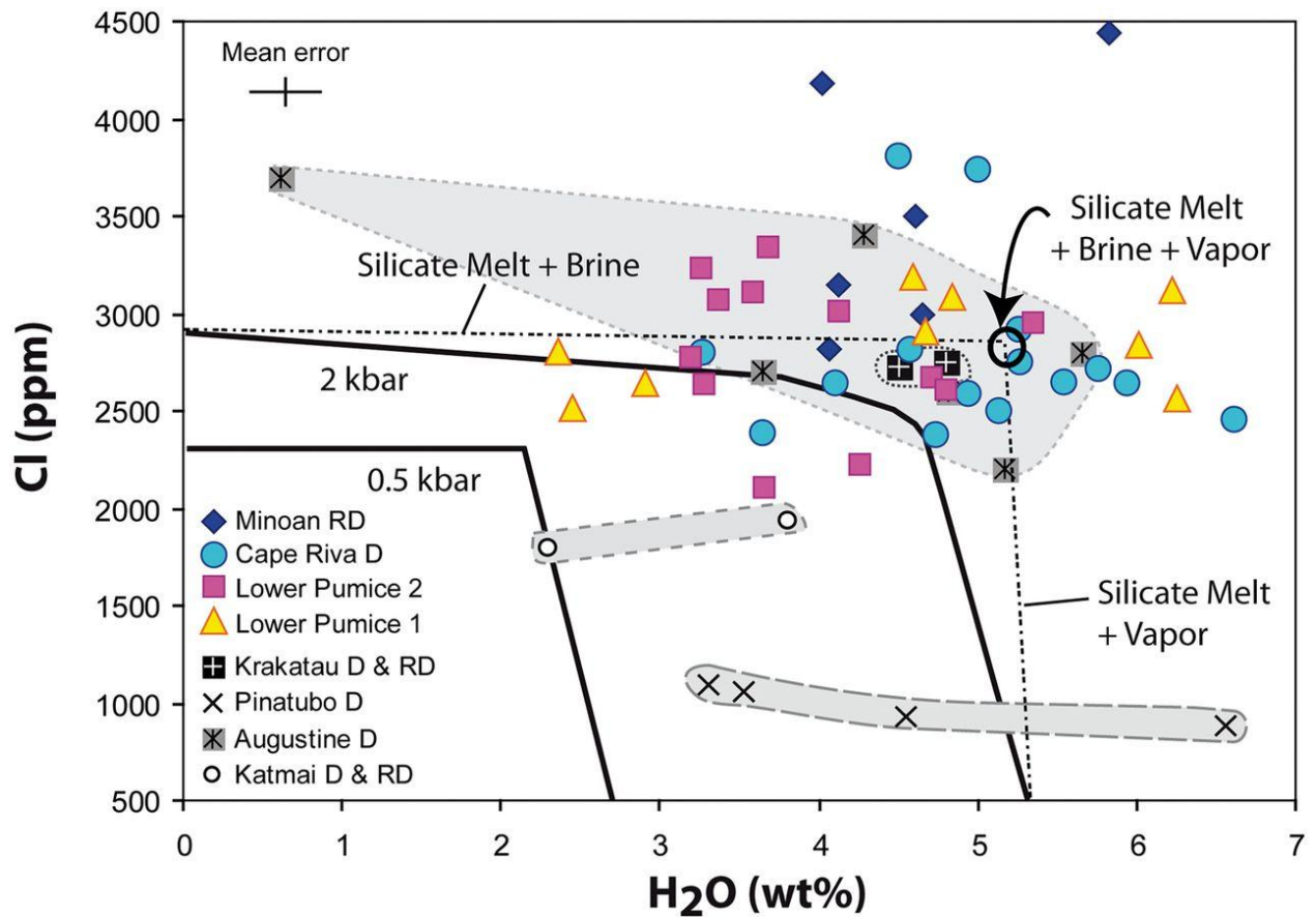
Figure 16. Chlorine (ppm) versus \text{H}_2\text{O} (wt%) contents dissolved in melt inclusions of plagioclase and pyroxene phenocrysts from the Minoan, Cape Riva, Lower Pumice 2 and Lower Pumice 1 silicic magmas. They are compared with melt inclusions of other silicic arc magmas from Augustine and Katmai volcanoes (Alaska; Hildreth, 1983; Westrich et al. , 1991; Hammer et al. , 2002; Roman et al. , 2006), Krakatau (Indonesia, Mandeville et al. , 1996) and Pinatubo (Philippines, Gerlach et al. , 1996). D and RD refer to the whole-rock composition: D = dacite, RD = rhyodacite.
