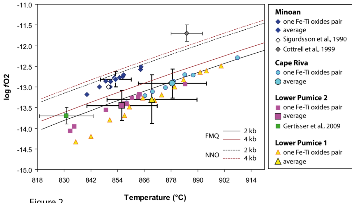
Figure 2. Oxygen fugacity ( \log fO_2 ) versus temperature ( ^{\circ}C ) calculated from Fe-Ti oxides from silicic pumices of the Minoan, Cape Riva, Lower Pumice 2 and Lower Pumice 1 eruptions (calculations performed with Stormer, 1983, and Andersen & Lindsley, 1985). All the ilmenite and magnetite pairs used for calculation are in equilibrium, according to their Mg/Mn ratios (Bacon & Hirschmann, 1988). They are touching and non-touching pairs included in the same pyroxene crystal or, touching pair in the groundmass. Previously published T - fO_2 estimates for the Minoan (Sigurdsson et al. , 1990; Cottrell et al. , 1999) and the LP2 (Gertisser et al. , 2009) eruptions are also shown. The FMQ and NNO oxygen fugacity curves were calculated for 2 and 4 kbar using Frost (1991).
