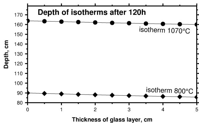
Figure 19. Effect of a glassy crust up to 5 cm thick on the depth of the 800°C and 1070°C isotherms in a lava flow emitted at a temperature of 1140^\circ\text{C} after 120 h of cooling, with the glass layer installed at t = 0 . A heat transfer coefficient ( h_{\text{cref}} ) value of 500 \text{ W m}^{-2} \text{ K}^{-1} and thermal conductivities of 1.25 for the glass and 2.5 \text{ W m}^{-1} \text{ K}^{-1} for the lava have been set for these calculations.
