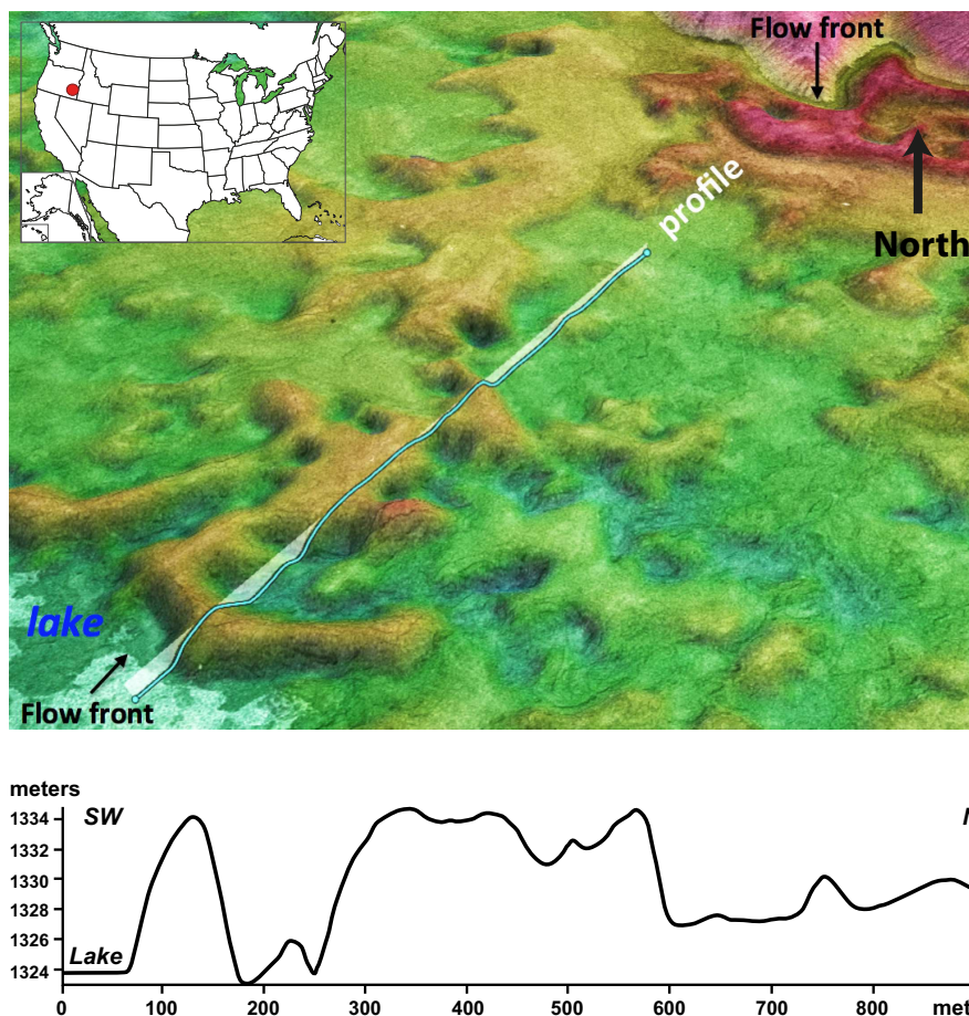
Figure 6. Blowout on the Southwestern flow front of the Jordan Crater inflated lava field, Oregon. (a) A 3-D view of aerial photographs draped on the Digital Elevation Model (DEM) and (b) topographic cross section across a pressure ridge (location is indicated on Figure 4).
