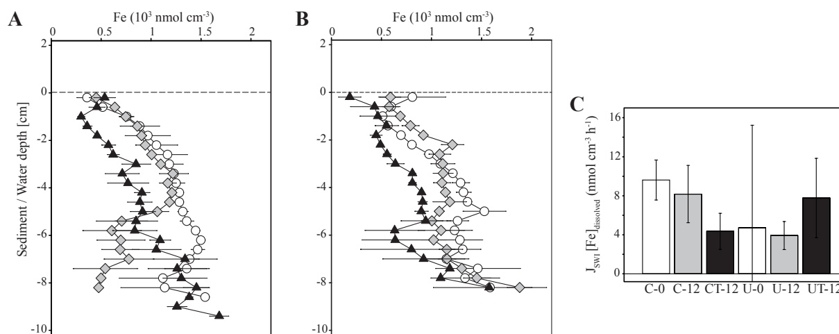
Figure 3. Dissolved total Fe concentration profiles in uncontaminated (A) and U-spiked sediment (B) in the different treatments: at initial conditions [C-0] and [U-0] (○) and after 12 days without [U-12] (◇) or with [UT-12] (▲) T. tubifex worms in the sediment. The bar chart (C) indicates the corresponding integrated outward diffusive fluxes at the sediment–water interface estimated using PROFILE software. Means \pm SD ( N = 3 ). No significant difference was detected between treatments.
