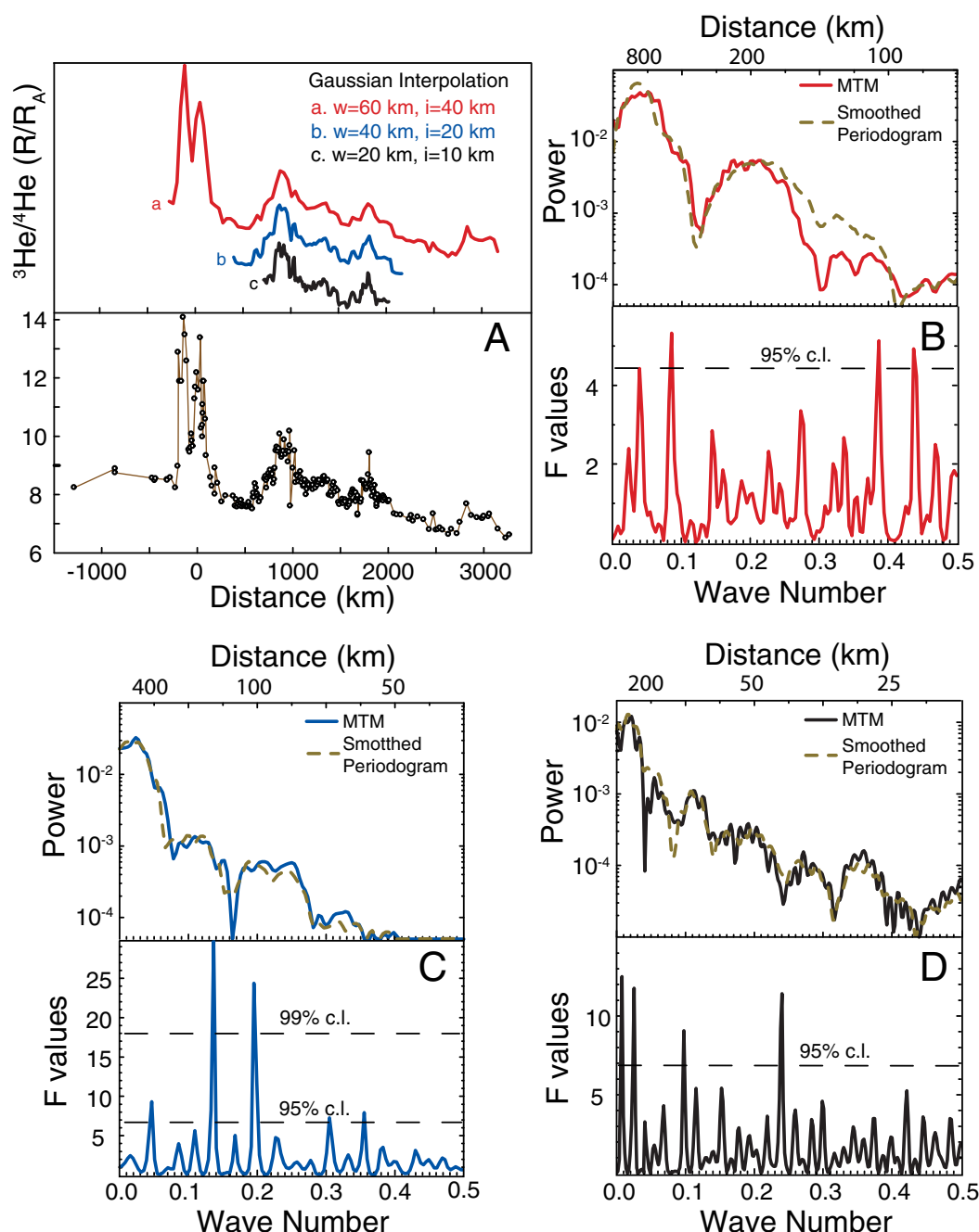
Figure 10. MTM analysis of the SEIR He isotope variations. (a) Gaussian interpolation of the variations. The data series was treated in three different ways. In treatment (a), the He isotope data were interpolated along-axis between -300 and +3140 km, at an interval ( i ) of 40 km using a Gaussian filter having a half-width ( w ) of 60 km. The total number of interpolated locations ( n ) is 87 . The MTM applied to treatment (a) shown here utilized five tapers. In treatment (b), the along-axis distance ranged from 380 to 2140 km, w = 40 km, i = 20 km, and n = 89 . The MTM applied to treatment (b) shown here utilized three tapers. In treatment (c), the along-axis distance ranged from 700 to 2010 , w = 20 km, i = 10 km, and n = 132 . The MTM applied to treatment (c) shown here utilized three tapers. (b–d) show the spectrum estimates from the MTM, and the corresponding confidence levels from the computed F-test values. The smoothed periodograms for the same data treatments are shown for comparison. Wave number range is from zero to the Nyquist limit (= sampling interval divided by 0.5 ), corresponding to 80 , 40 , and 20 km for series a, b, and c, respectively.
