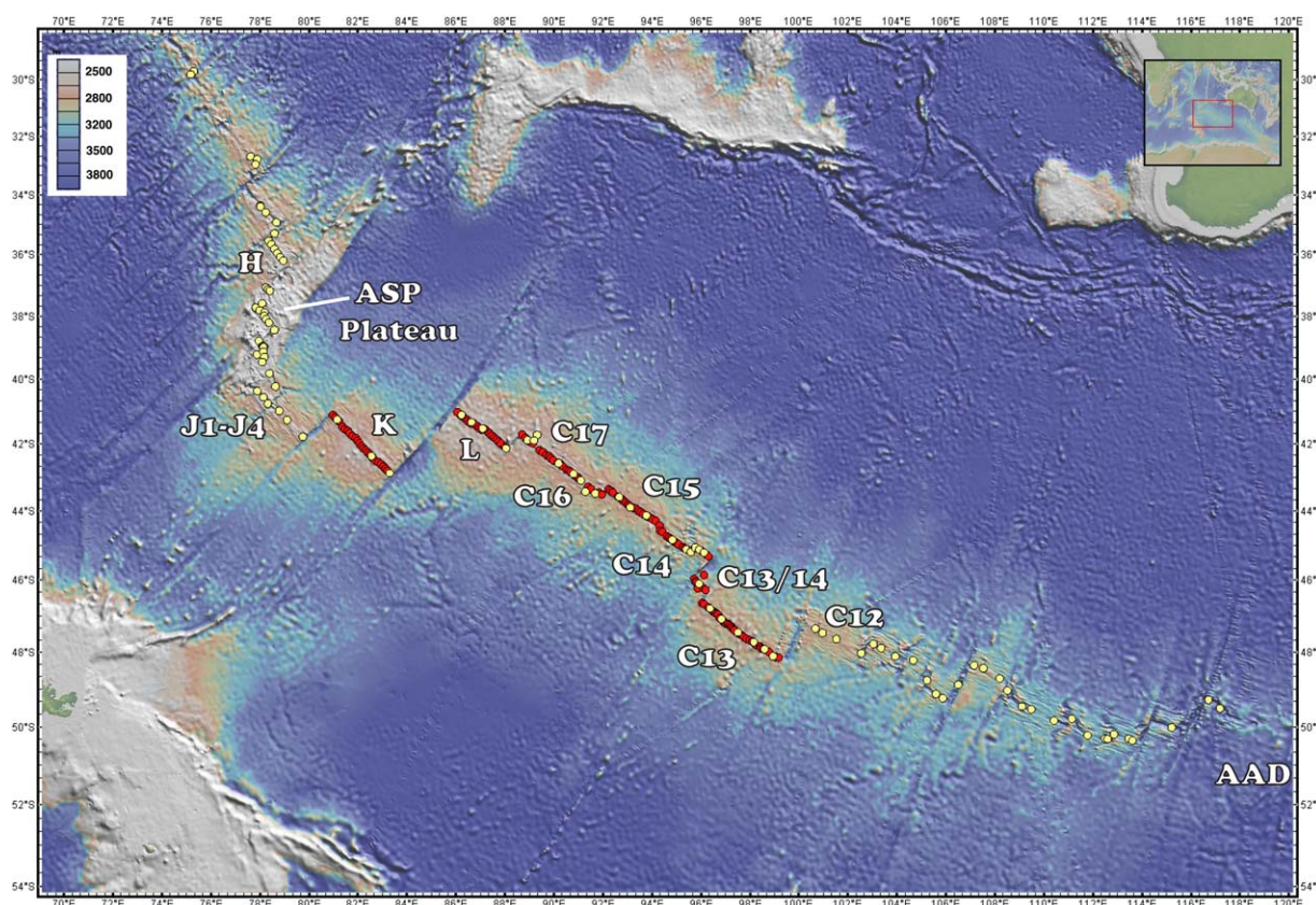
Figure 1. Location map of basalt glasses from the Southeast Indian Ridge analyzed for He isotopes. Individual ridge segments, the Amsterdam-St. Paul (ASP) Plateau, and the Australian-Antarctic Discordance (AAD) are indicated. Red circles are the GEISEIR I and II sample suites from this study. Other samples in yellow have ^3\text{He}/^4\text{He} data reported in Graham et al. [1999, 2001], Mahoney et al. [2002], and Nicolaysen et al. [2007]. The base map was made using GeoMapApp ( http://www.marine-geo.org/geomapapp ), which is supported by the National Science Foundation and internal funding from Lamont-Doherty Earth Observatory.
