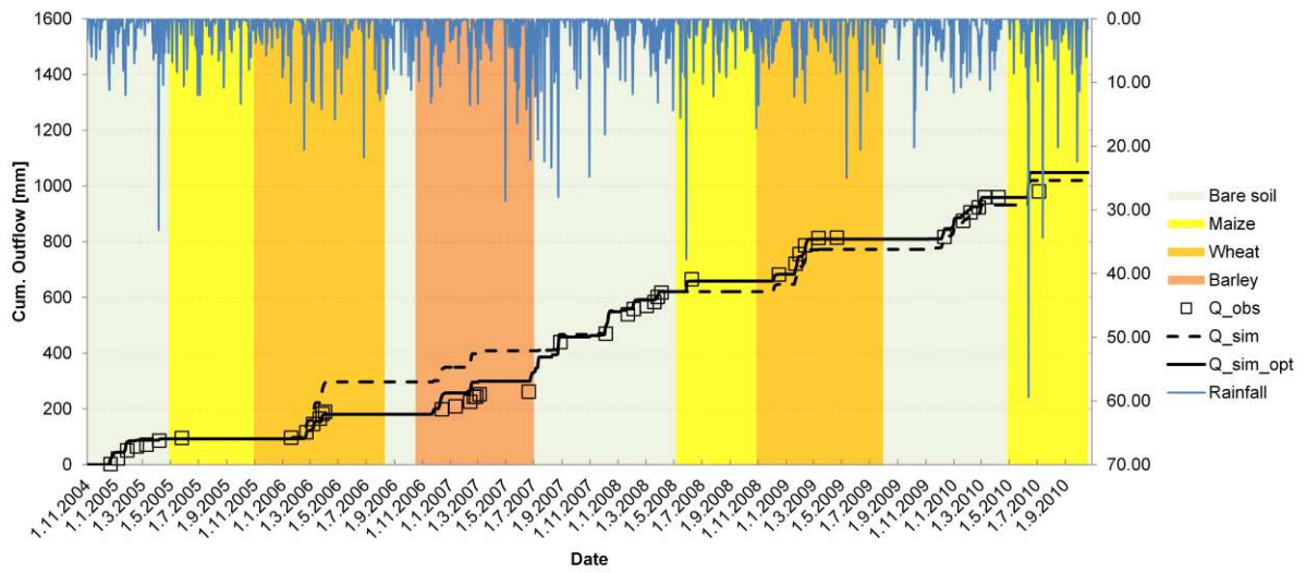
Fig. 5. Observed (symbols) vs simulated (line) cumulative lysimeter outflow using calibrated soil hydraulic parameters before ( Q_{sim} ) and after ( Q_{sim\_opt} ) LAI optimization.
