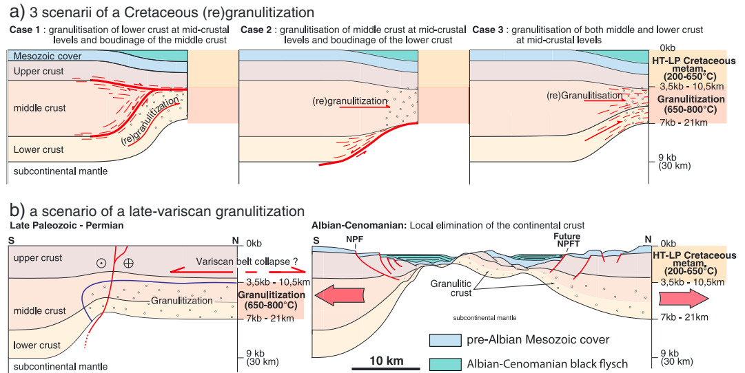
Figure 9. Cartoons showing different hypothesis for the origin and significance of the granulites exposed in the NPZ.
