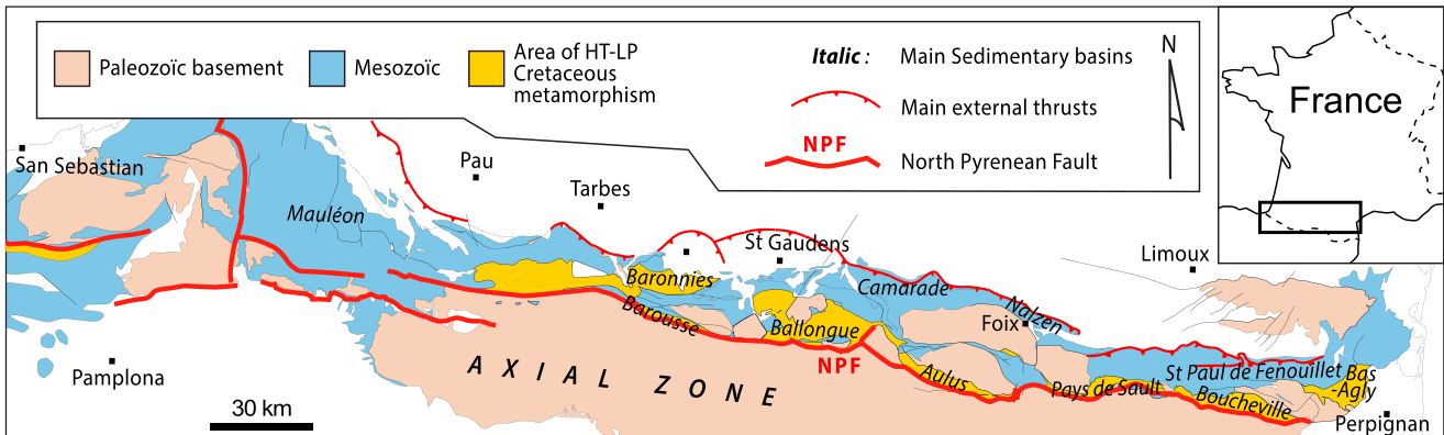
Figure 1. Simplified geological map of the northern Pyrenean belt. The area between the North Pyrenean Fault (NPF) and the main external thrusts is known as the North Pyrenean Zone (NPZ).
