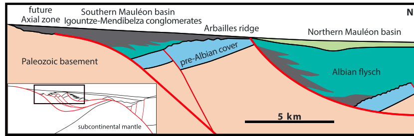
Figure 3. Reconstructed profile across the Mauléon basin and Arbailles ridge (after Masini et al. [2014]).
