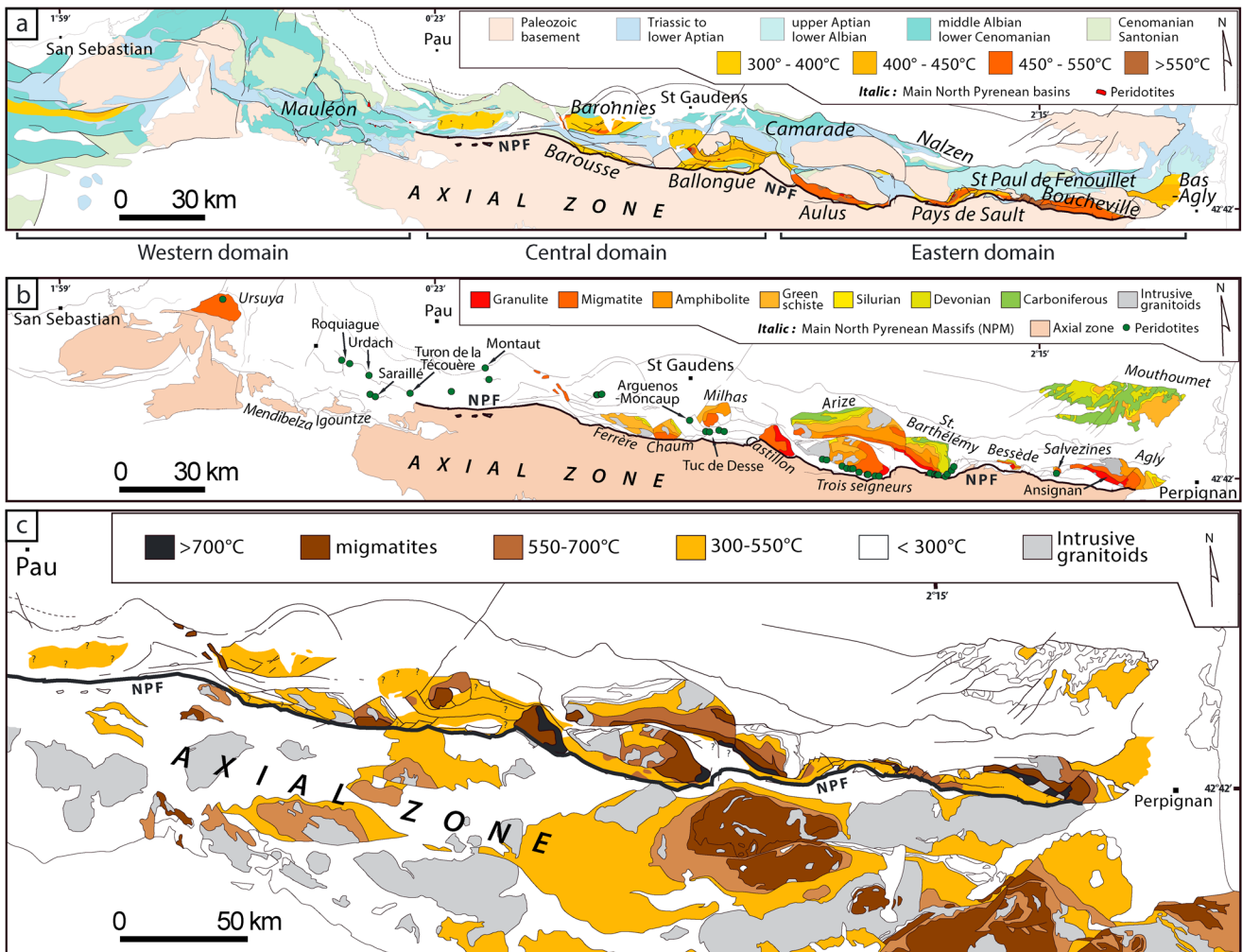
Figure 2. Maps of the Pyrenean belt compiled from various data [Choukroune and Séguret, 1973; Golberg and Leyreloup, 1990; BRGM and IGME, 1998; Jammes et al., 2009] and from the 1/50,000 geological maps of the BRGM. (a) Isotemperature map of the NPZ [paleotemperatures are compiled from Golberg and Leyreloup, 1990; Clerc, 2012; Vauchez et al., 2013]. (b) Simplified geological map of the NPZ massifs with location of the outcropping peridotite bodies. (c) Isotemperature map of both the Paleozoic basement and the Mesozoic cover for the entire northern Pyrenees, including the Axial Zone.
