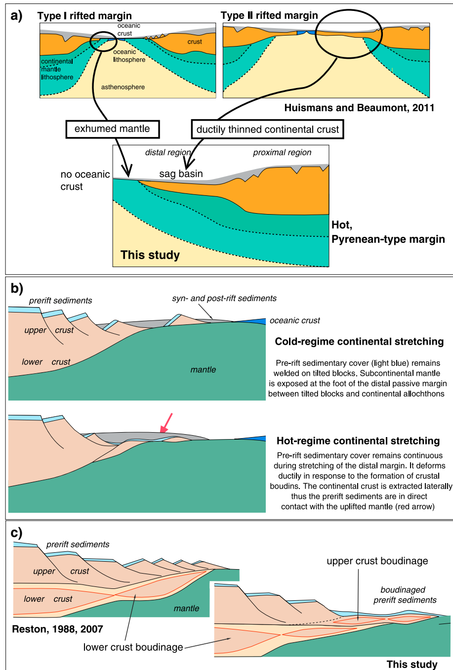
Figure 7. Cartoons illustrating the main differences between the model of hot continental stretching proposed in this article and some models of passive margin formation from the literature. (a) The model of hot passive margin established from the Pyrenean case (lower sketch) includes fundamental characteristics from both margins of type I and II by Huismans and Beaumont [2011]. (b) The lower cartoon represents an idealized section of a passive margin, which originated under the conditions of hot-regime stretching. It strongly differs from a cold margin, which is characterized by the formation of continental allochthons. (c) Lower crustal boudinage is proposed in a model by Reston [2007]. Our study allows us to propose an alternative model in which the upper crust is also boudinaged.
