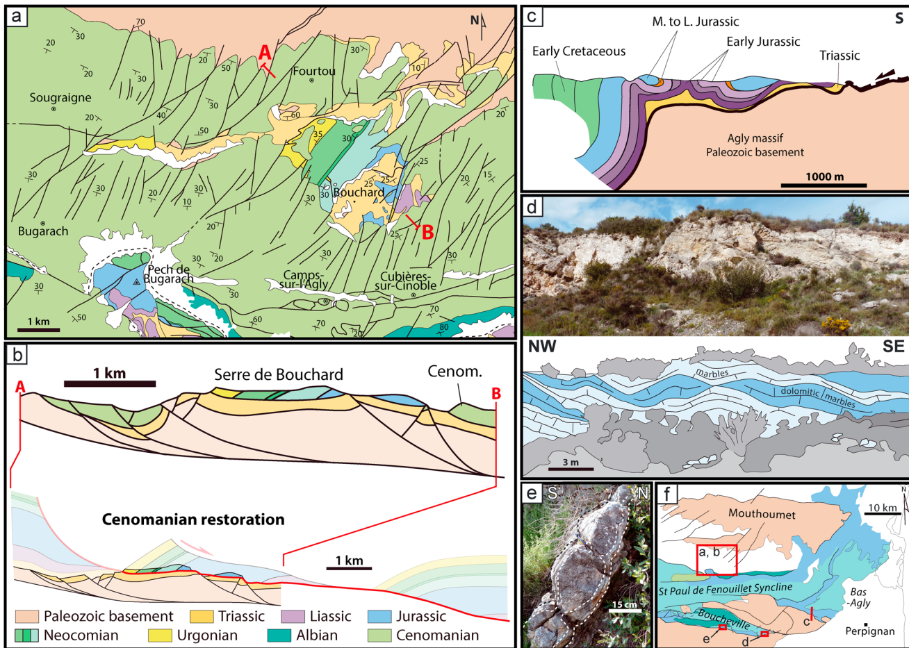
Figure 4. (a) Geological map of the southern border of the Mouthoumet massif in the Boucharde-Fourtou area (after Crochet et al. [1989]). (b) A cross section along the A-B profile (after Bessière [1987]) and its Cenomanian restoration showing decollement and tilting of the Mesozoic cover are proposed. (c) Decollement, basal truncation, and boudinage of the prerift Mesozoic cover of the Agly massif (after Vauchez et al. [2013]). Field illustrations of this boudinage in Mesozoic marbles in the (d) Belesta (coordinates 42°43'19N–02°35'48E) and (e) Sournia areas (coordinates 42°43'19N–2°26'49E). Elements a, b, c, d, and e of the figure are localized in f (same legend as Figure 2a).
