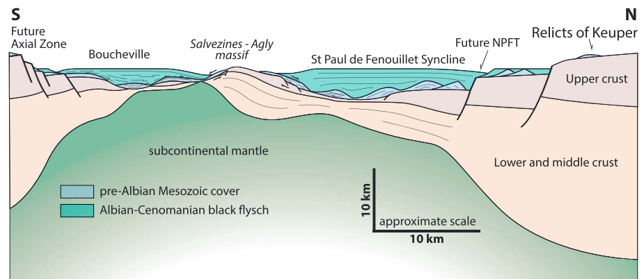
Figure 5. A conceptual reconstructed section across the European paleomargin of the eastern Pyrenees (after a balanced cross section of Clerc [2012]). The section includes the Boucheville, Bas-Agly, and Saint Paul de Fenouillet Cretaceous basins. It shows the Salvezines continental boudin. Thick lines represent faulted contacts.
