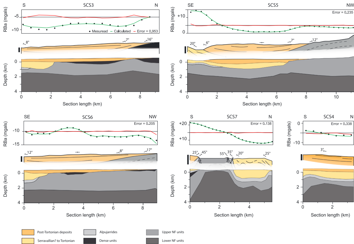
Figure 9. Total gravity anomaly, shallow field-based cross section and corresponding 2-D model constructed for the five cross sections called SCS3 to SCS7. The gravity modeling of these cross sections is equal to that detailed in the text for the basin-scale SCS1 cross section. Vertical exaggeration = 2; see Figure 7 for location.
