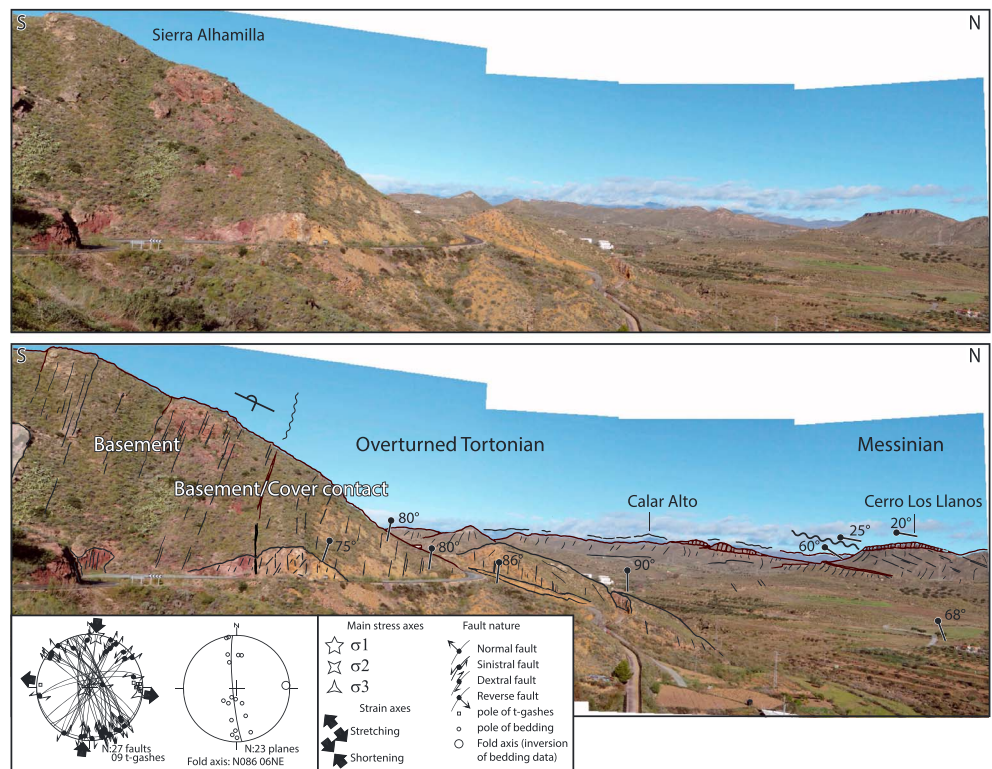
Figure 4. Evidences of upper Tortonian compressive tectonic. Panoramic view of the southern folded boundary of the Sorbas basin East of Lucainena de las Torres (see location in Figure 2). Here the metamorphic basement describes a north verging asymmetric fold with an overturned steep-dipping forelimb. Tortonian series, separated from the basement by an unconformity, display a rather continuous growth-strata structure forming a recumbent syncline. Fault-slip data inversion indicates a N-S maximum compression direction [ \sigma_1 ].
