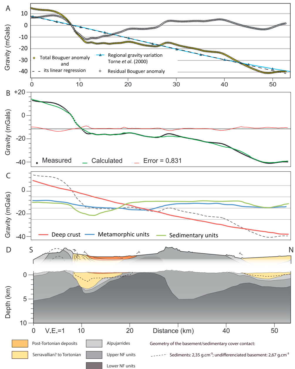
Figure 8. Two-dimensional gravity profile treatment. (a) Comparison between the measured total Bouguer anomaly (yellow diamond shape) and the regional gravity deviation exposed in Tome et al. [2000] of the N-S regional cross-section (SCS1). White diamond-shaped points represent the calculated residual Bouguer anomaly profile (see text for details). (b) Superposition of the 2-D gravity model anomaly (green curve), calculated from the density summarized in Table 1, with the measured total Bouguer anomaly (black dots). The red curves correspond to the difference between the modeled gravity anomaly and the measured one. (c) Deconvolution of the measured gravity signal (black dashed line) showing the combined effects of the deep structures of the crust and more particularly the Moho geometry (red curve); the upper crust structure of the outcropping metamorphic units (blue curve) and the shape and thickness of the sedimentary basins (green curve). (d) Shallow field based cross section and interpretation of the modeled 2-D gravity anomaly across the Sorbas basin. Note the strong asymmetry of the sedimentary depocenter.
