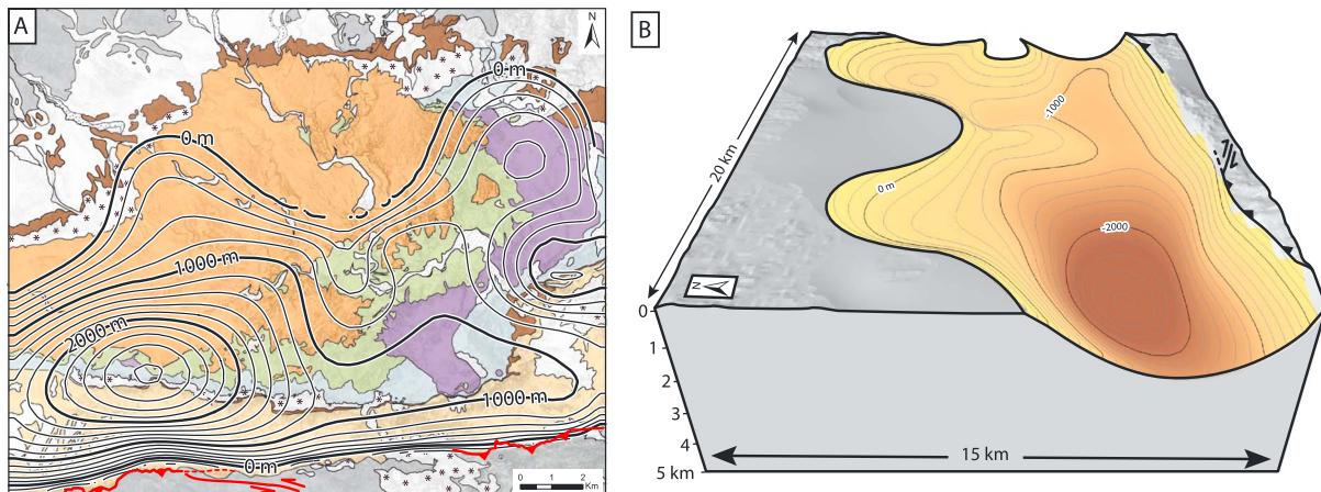
Figure 10. Basin floor 3-D geometry. (a) Isodepth curves of the base of the Tortonian deposits are plotted over the geological map of the modeled area. The depth is indicated in meters below sea floor. (b) Three-dimensional oblique view of the base of the Sorbas basin. Vertical exaggeration = 3.
