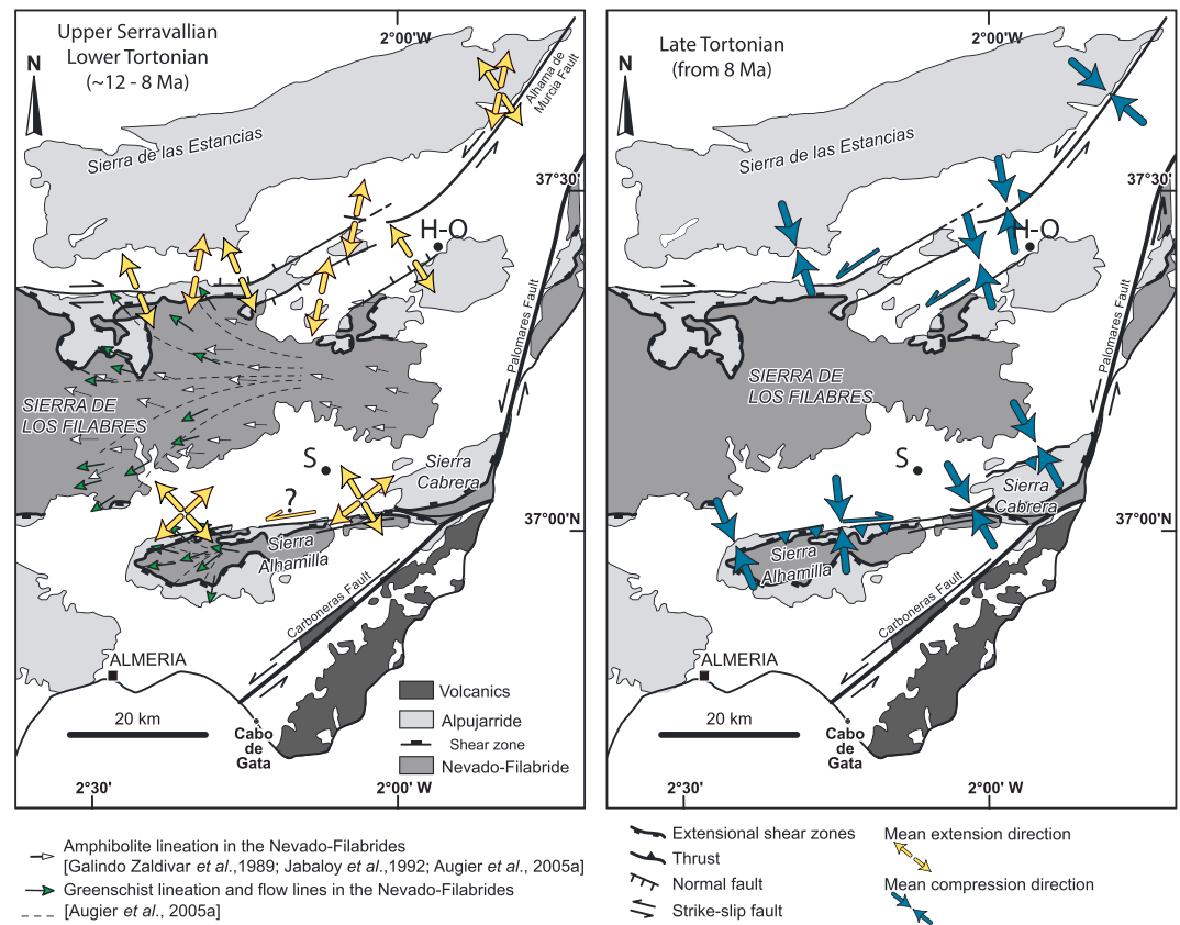
Figure 12. Simplified tectonic map showing average upper Serravallian-lower Tortonian extension directions and average upper Tortonian compressive directions of the southeastern part of the Internal Zones of the Betic Cordillera. Stretching direction and associated sense of shear for the Nevado-Filabride complex are synthesized from [Galindo-Zaldívar et al. , 1989; Jabaloy et al. , 1992; Augier et al. , 2005a]. Extension and compression directions shown in the Huércal-Overa basin are derived from Meijninger [2006] and Augier et al. [2013].
