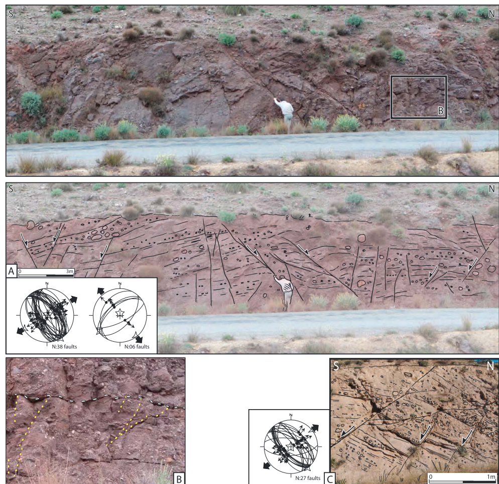
Figure 5. Field evidences of extensional deformation affecting upper Serravallian to upper Tortonian sediments, (location in Figure 2). (a) Uninterpreted and interpreted panorama of lower Tortonian reddish conglomerates affected by two sets of small-scale normal faults: a dominant approximately N140E and a subordinate approximately N30E conjugate sets of normal faults. (b) A close-up view of syndimentary normal faults affecting sandy to microconglomerate intervals and interrupted by a coarse-grained conglomerate. (c) Upper Tortonian marine sediments affected by a N140E oriented set of small-scale normal faults.
