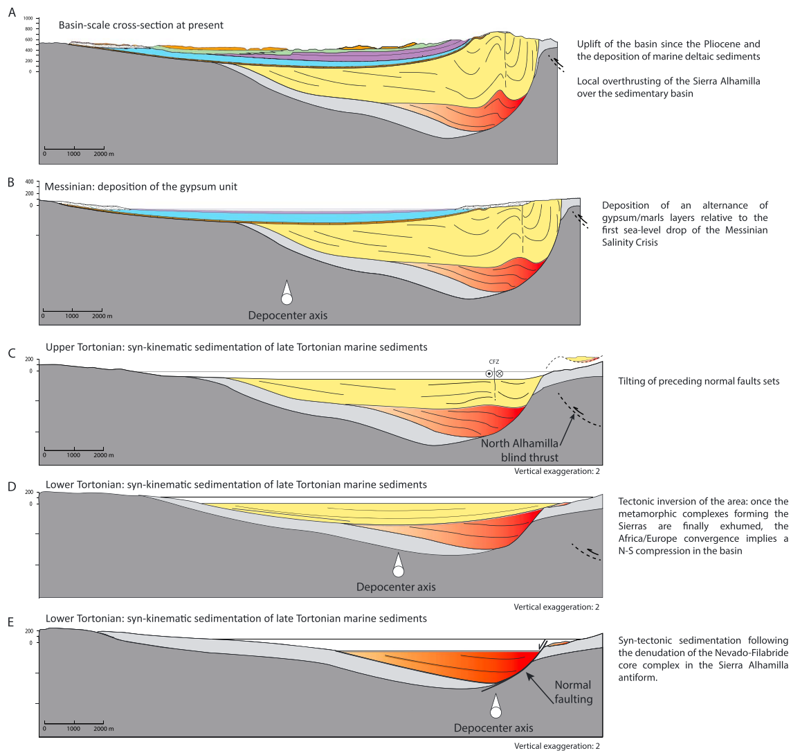
Figure 13. Interpretative N-S cross sections of the Sorbas basin representing its evolution from (a) the present to the deposition of (b) Messinian evaporites, (c) the late Tortonian syntectonic sedimentation of turbidites, and (d) the period of tectonic inversion postdating the extensive deformation during (e) the upper Serravallian to lower Tortonian.
