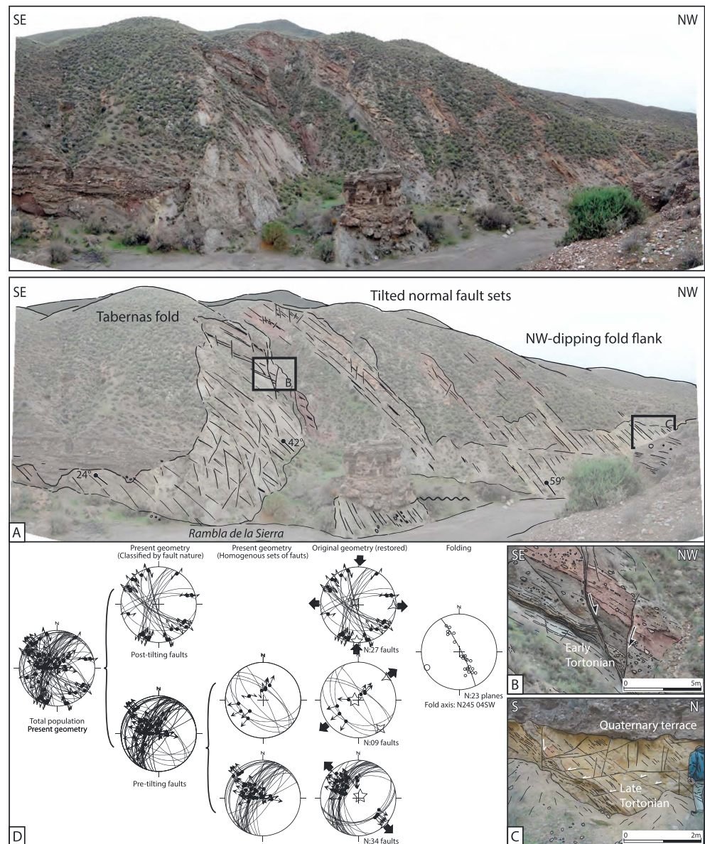
Figure 6. Geometrical relationships existing between the upper Serravallian-Tortonian extensional deformation and the upper Tortonian inversion. (a) Uninterpreted and interpreted panoramic view of the northern flank of the so-called Taberns fold [Ott d'Estevou and Montenat, 1990] showing (b) the presence of tilted normal faults affecting the lower Tortonian deposits and also (c) the upper Tortonian marine sediments. (d) The decomposition of the total heterogeneous fault population into homogeneous, cogenetic fault populations shows the presence of two subhorizontal extensional regimes with N50E and N140E minimum compression direction ( \sigma_3 ) that predate inversion tectonics visible at all scales from microfaults to large-scale folding.
