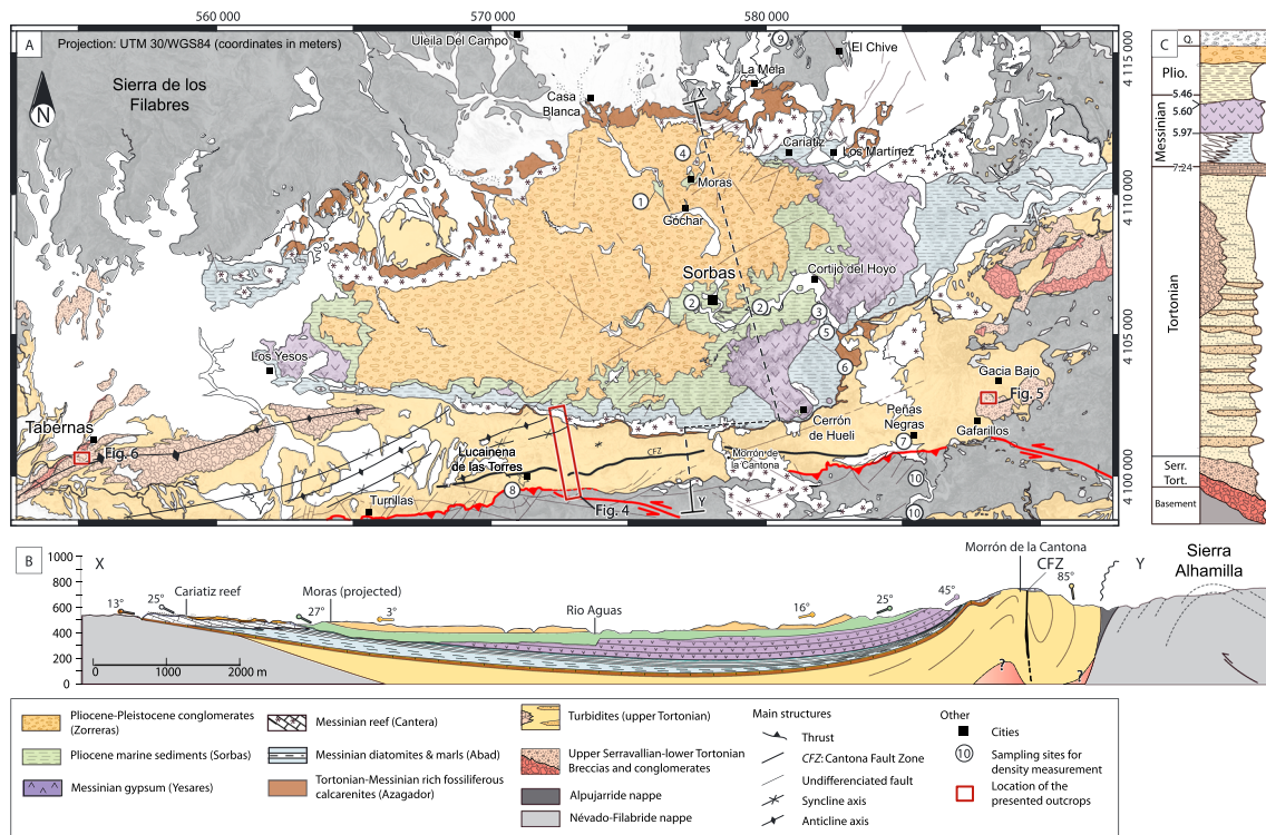
Figure 2. Structure and stratigraphy of the Sorbas basin. (a) Geological map of the Sorbas basin, modified from Ott d'Estevou and Montenat [1990] and García Monzón et al. [1974]. Projection UTM Zone 30 (WGS84 ellipsoid). (b) Synthetic N-S cross-section X-Y representing the main architecture of the Sorbas basin (location in Figure 2a). (c) Synthetic stratigraphic log of the Sorbas basin. Modified after Montenat and Ott d'Estevou [1977], Ott d'Estevou and Montenat [1990], Krijgsman et al. [1999], Krijgsman et al. [2001], and Manzi et al. [2013].
