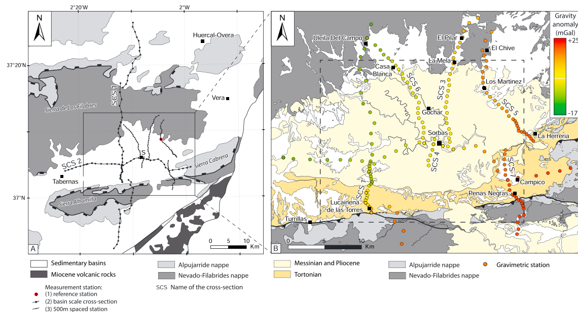
Figure 7. (a) Simplified geological map showing gravimetric cross sections realized across the basin. Red circle represents the reference station. (b) Location of the gravimetric stations and gravity anomaly plotted over the geological map of the Sorbas Basin. All measurement stations are represented by small circles colored in function of their relative Bouguer anomaly (see the color bar in the upper right corner). The dashed border rectangle represents the extension of the modeling box used to model in 3-D the sediments/basement interface at depth.
