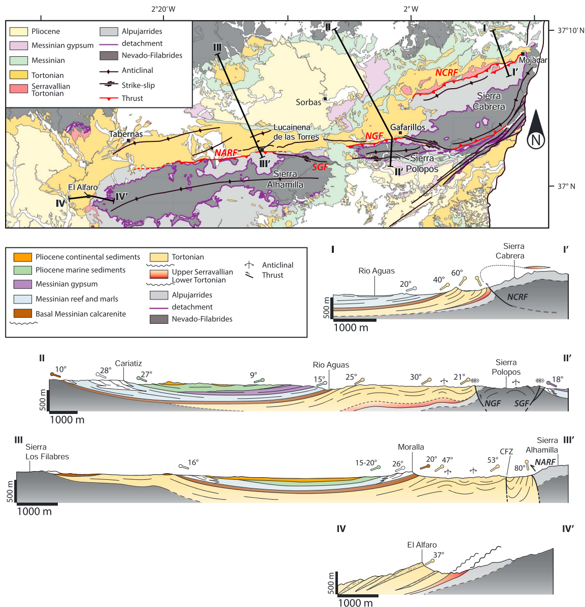
Figure 3. Simplified geological map showing the four main faults accommodating the deformation along the Sierra Alhamilla, Sierra Polopos, and Sierra Cabrera: from East to West, the North Cabrera reverse fault (NCRF), the North Gafarillos fault (NGF), the South Gafarillos Fault (SGF), and the North Alhamilla reverse fault (NARF). Four cross sections, orthogonal to the sediments/basement contact, present the geometry and architecture of the sedimentary units with respect to the metamorphic ridges (location of cross sections in the geological map). See text for more details.
