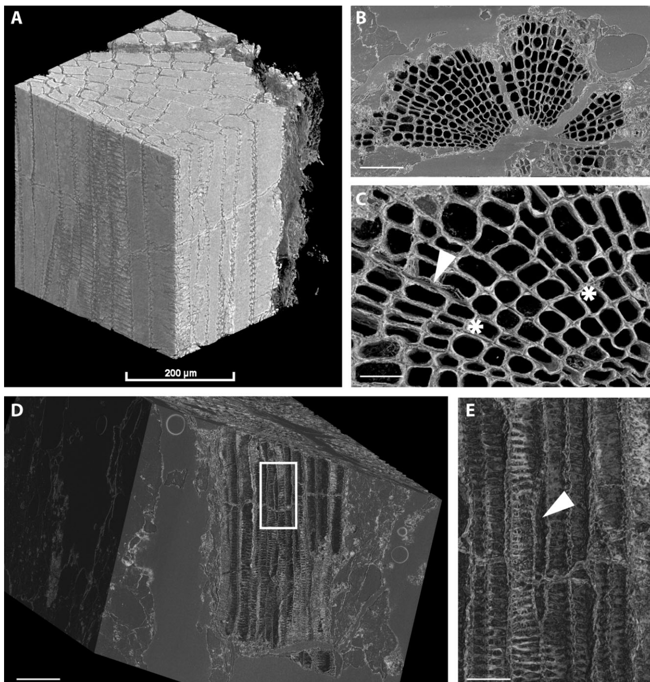
Figure 4. Armoricaphyton chateaupannense . Specimen CSD-07F-01: holotype. High-resolution propagation phase contrast X-ray synchrotron microtomography (PPC-SRμCT) of c. 407-million-year-old fossil wood preserved in the mineral pyrite (FeS 2 ). A, Three-dimensional representation of part of the pyritized axis, which has been virtually trimmed to a cubic volume. Xylem tracheids are visible in longitudinal, radial and transverse sections. B, Transverse section of part of the xylem embedded in a shale matrix. In this image, the mineral pyrite has been virtually dissected out, leaving behind the organic framework of the tracheid cell walls. C, Higher magnification of (B). Tracheids are generally rectangular in transverse section. In several places, two xylem cell rows emanate from a single row (asterisks); single-walled space interpreted as ray (arrow). D, Longitudinal tangential section of part of the xylem in which the pyrite has been virtually dissected. E, Detail of the framed area from (D); secondary xylem showing tracheids and a one-cell ray. A double wall (consisting of the secondary walls of each tracheid) is visible between adjacent tracheids, whereas a single wall occurs between ray (arrow) and tracheid cells. The wall of the ray was not preserved. Scale bars: 300 μm (B); 50 μm (C, E); 150 μm (D).
