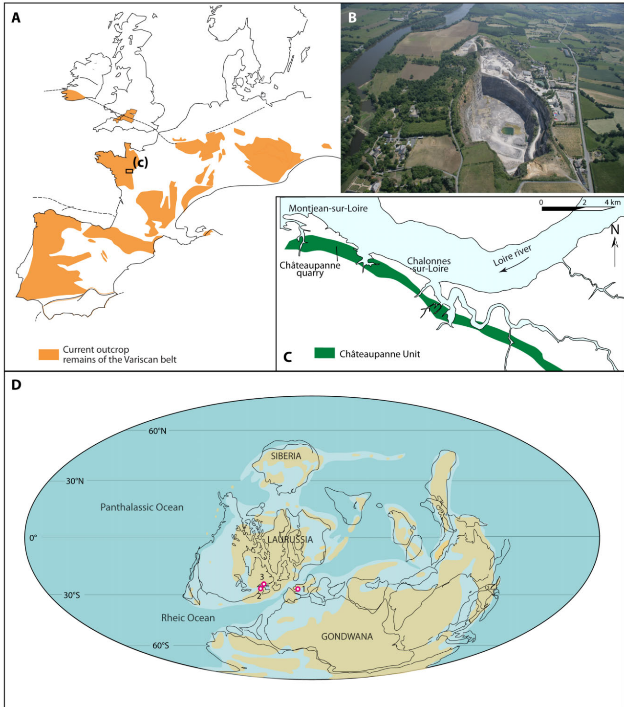
Figure 1. Location of the study area and palaeogeography. A, Location [rectangle expanded in (C)] of the study area in the European Variscan Belt and the Armorican Massif. B, The Châteaupanne Quarry (aerial view) with permission of R. Jospin. C, Lower Devonian deposits from the Anjou area (Châteaupanne Unit). D, Early Devonian palaeogeography (after Scotese, 2001, modified). Continental land masses are indicated in light brown and shelves in light blue; the fine line drawing indicates the outlines of the present continents. Geographical relationships of the sites of the three early woody plants: 1, Anjou area in the Armorican Massif (western France); 2, New Brunswick, Canada; 3, Gaspé, Canada.
