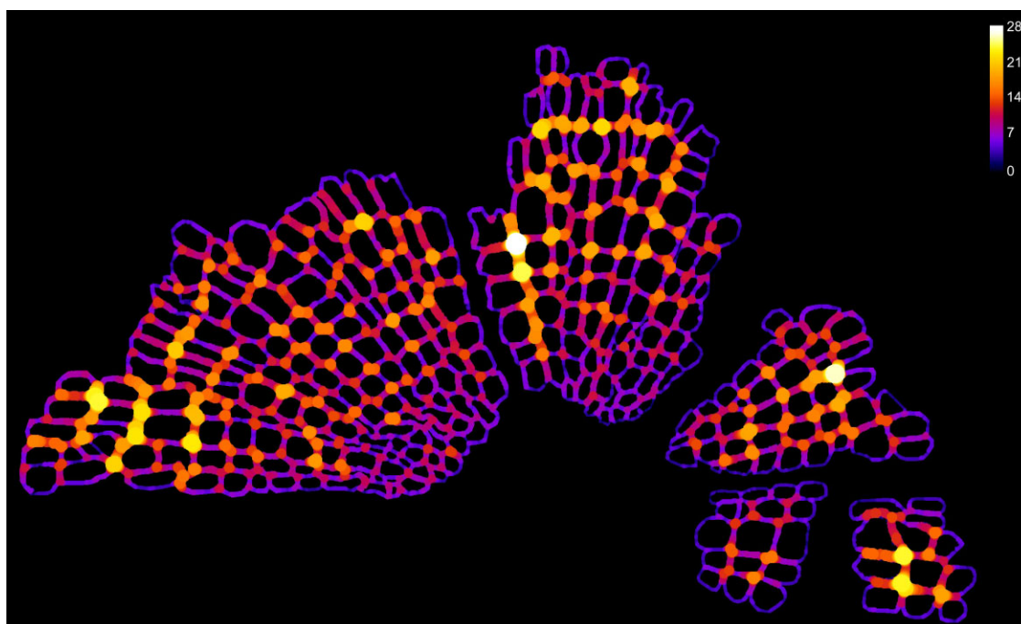
Figure 6. Transverse section of xylem cell lumens of Armoricaphyton chateaupannense extracted from the propagation phase contrast X-ray synchrotron microtomography (PPC-SR \mu CT) volume to map cell dimensions (CSD-07F-01). The geometrical parameters (i.e. area, diameter, perimeter) of each tracheid were measured to evaluate the individual hydraulic conductivity using the hydraulic radius approximation. The cell wall thickness was mapped using the Hildebrand algorithm in order to calculate the thickness-to-span ratio (t/b)^2 , which reflects the sensitivity of the cells to transverse mechanical buckling under negative pressure. The brighter the colour, the thicker the double cell wall ( \mu\text{m} scale).
