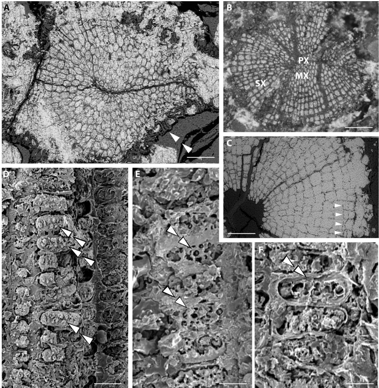
Figure 3. Anatomy of the axes. Specimens CSD-06C-04, CSD-06A-01: paratypes. A–C, Transverse sections of pyritized axes. A, Axis in which the secondary xylem is not well developed. A layer of large thick-walled cells (sterome) is visible in the outer cortex (arrows) [scanning electron microscopy (SEM), backscatter electrons] (Specimen CSD-06C-04). B, Axis showing both primary and secondary xylem; MX, metaxylem; PX, protoxylem; SX, secondary xylem (microscopy using polarized light source) (Specimen CSD-06A-01). C, Axis showing a primary xylem area (not preserved) surrounded by rows of ten radially aligned tracheids of secondary xylem. Some tracheids have a smaller radial diameter in places within the wood (arrows) (SEM, backscatter electrons) (Specimen CSD-06C-02). D–F, P-type tracheids fractured in longitudinal section to show aspects of the cell wall in different planes of fracture (SEM) (Specimen CSD-06A-01). D, Pyritized casts of the interior chambers of the scalariform bordered pits (arrows). E, Coalified remains of pit-closing perforated sheet in two partly visible pit fields (arrows). F, Row of scalariform bordered pits. The pit chamber cast has fallen out of one to reveal organic remains of the pit borders and part of the pit-closing perforated sheet (arrow). Scale bars: 200 \mu\text{m} (A, C); 300 \mu\text{m} (B); 14 \mu\text{m} (D, E); 7 \mu\text{m} (F).
