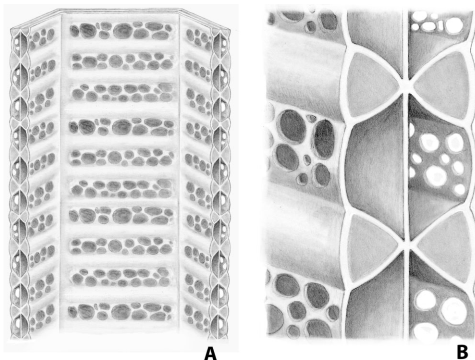
Figure 5. P-type tracheid. A, Reconstruction of a tracheid. Drawing of cut-away longitudinal section, showing interior of cell ( \times 800 ). Cell with scalariform bordered pits with overarching pit borders and a characteristic perforated sheet of secondary wall material that overlies the pit apertures. B, Detail of tracheid cell wall construction ( \times 2500 ). The cell wall comprises an inner layer facing the cell lumen, pit chambers, and an inner layer within the scalariform bars. The scalariform pit apertures are covered with a perforated sheet. Drawing by Pollyanna von Knorring, modified after Kenrick & Crane (1997a).
