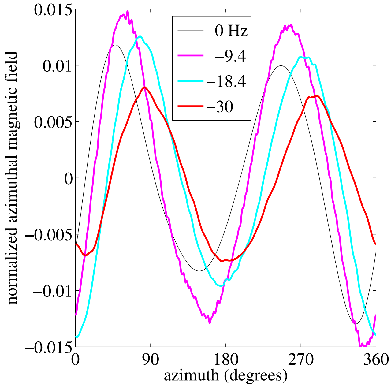
FIG. 2. (Color online) 2\pi -longitudinal motifs of the non-axisymmetric magnetic field recorded by a Hall magnetometer measuring B_\varphi for r = 0.79 at a latitude of -20^\circ , for increasing rotation rates of the inner sphere f = -9.4, -18.4 and -30 Hz. The magnetic field is normalized by B_o as indicated in table IV. The motif for f = 0 is computed from the scalar magnetic potential of the magnet.
