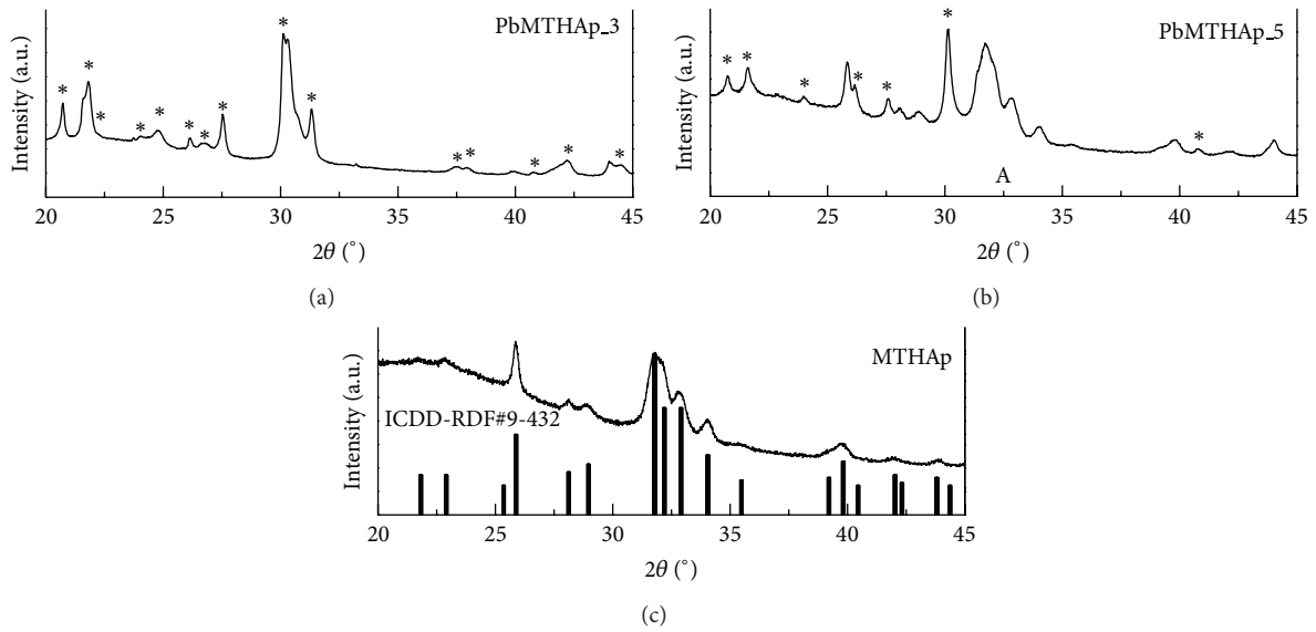
FIGURE 2: XRD patterns of hydroxyapatite coated with methyltrimethoxysilane before (MTHAp) and after the removal experiment of Pb^{2+} at pH 5 (PbMTHAp_5) and pH 3 (PbMTHAp_3). *—represent the packs associated with overlapping of Ca_{2.5}Pb_{7.5}(PO_4)_6(OH)_2 and Pb_2Ca_4(PO_4)_2(SiO_4) .
