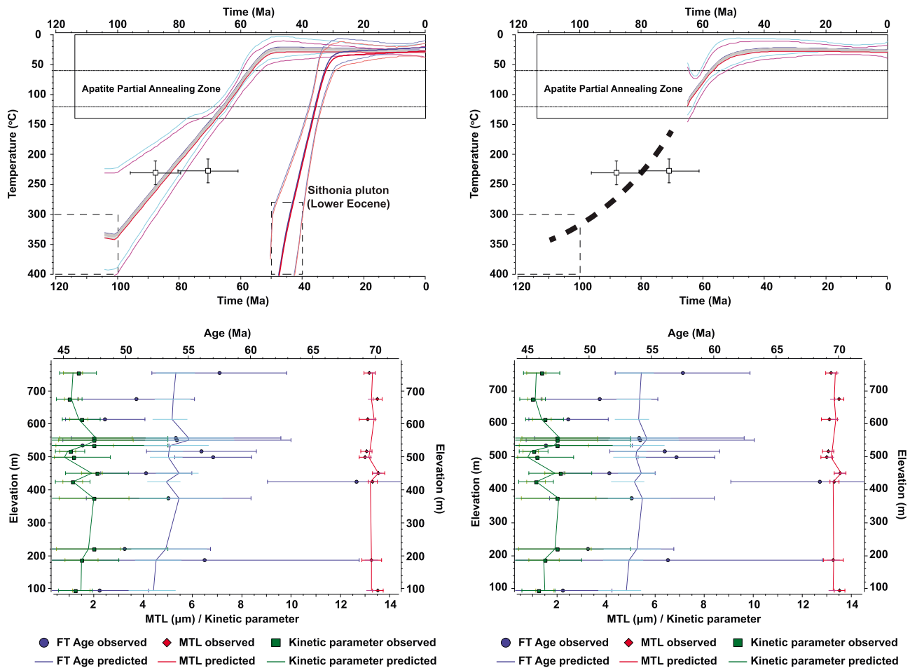
Figure 6. (top) The inferred expected model for 14 basement samples of the Vertiskos Unit treated as a vertical profile. The samples used are also shown in Figure 5 (SM54 excluded). The modeling approach is described in Gallagher et al. [2005b] and Gallagher [2012]. The model on the left originates from a constrained T-t area (dashed box; 350 \pm 50^\circ\text{C} at 120 \pm 20 Ma) based on the geological evidence and the available geochronology data (see text for details). The two empty squares correspond to the published ZFT age from the Vertiskos/Ograzden Units. For comparison, the result of the nonconstrained model is shown on the right. Red thick line is used for the thermal path of the hottest (lowest-elevation) sample (red thin lines 95% credible interval range) and blue thick line for the thermal path of the coolest (highest-elevation) sample (blue thin lines 95% credible interval range). Using the same modeling approach and the samples GR117, GR126, GR132, and GR134 from Hejl et al. [2010], we calculated, for comparison, the thermal path of the lower Eocene Sithonia pluton from the southern edge of the Chalkidiki peninsula (see Figure 1 for location). (bottom) The corresponding FT age (blue), mean track length (red), and kinetic parameter (green) predictions for the constrained and nonconstrained models are shown.
