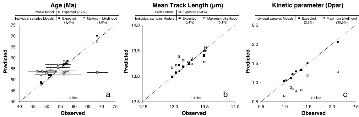
Figure 3. Observed versus predicted values of both the individual sample modeling (expected and maximum likelihood models) and the joint profile modeling approaches adopted here for (a) the age, (b) the mean track length, and (c) the sampled kinetic parameter. Error bars on the observed age are also shown for part of the data set. Numbers in parentheses is the average percentage deviation from the observed values for each data set.
