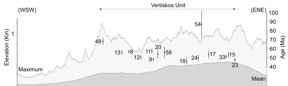
Figure 5. WSW-ENE trending swath elevation profile of the Chalkidiki Peninsula extracted from the ASTER Global DEM v2. The profile stretches from the Vardar-Axios basin to the Strymon basin (see Figure 1). The AFT ages for the samples used for the joint profile modeling approach are plotted, and the corresponding calculated apatite FT ages are read on the right vertical axis.
