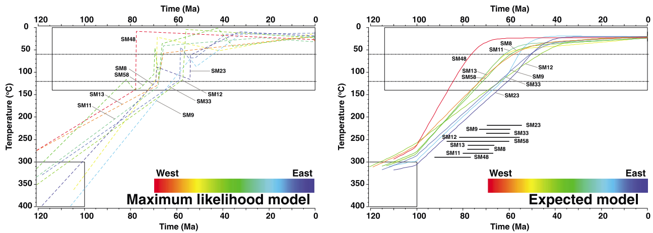
Figure 4. Compilation of the calculated (left) maximum likelihood and (right) expected models for nine samples of the Vertikos Unit that inferred using the individual samples approach (shown also in Figure 2). See Figure 1 for sample locations. For the expected model (right), the timing (2 sigma uncertainty included) that each individual thermal path (sample) crosses the high-temperature boundary of the apatite PAZ (~120°C) is also indicated.
