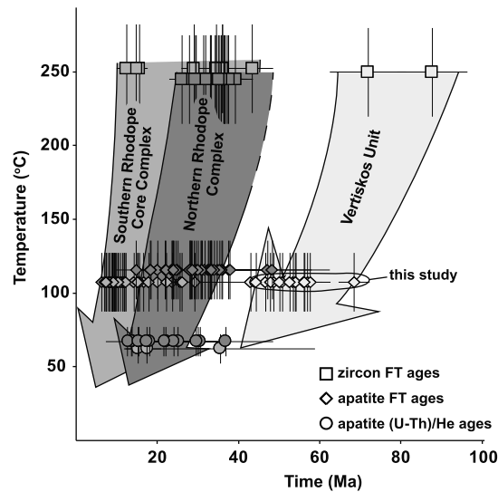
Figure 8. Simplified thermal paths (and data compilation) for the three tectonic domains shown in Figure 7. The available ZFT, AFT, and apatite (U-Th)/He ages are plotted against an “average” closure temperature (approximately 250, 110, and 60°C, respectively). The color fill of the three thermal paths (and the low-temperature data compilation) corresponds to the color fill of each of the three tectonic domains shown in Figure 7.
