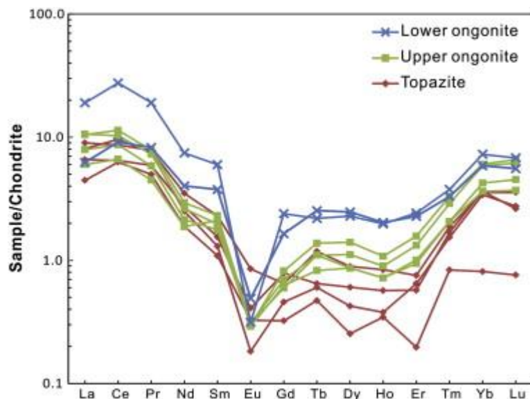
Fig. 5. : Chondrite-normalized REE patterns for the No. 431 dike (chondrite REE values from Anders and Grevesse, 1989).
