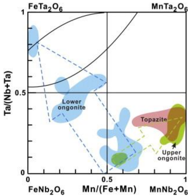
Fig. 12. : Fractionation trends of the columbite-group minerals and topazite from the No. 431 dike. Arrows indicate direction of compositional fractionation.
