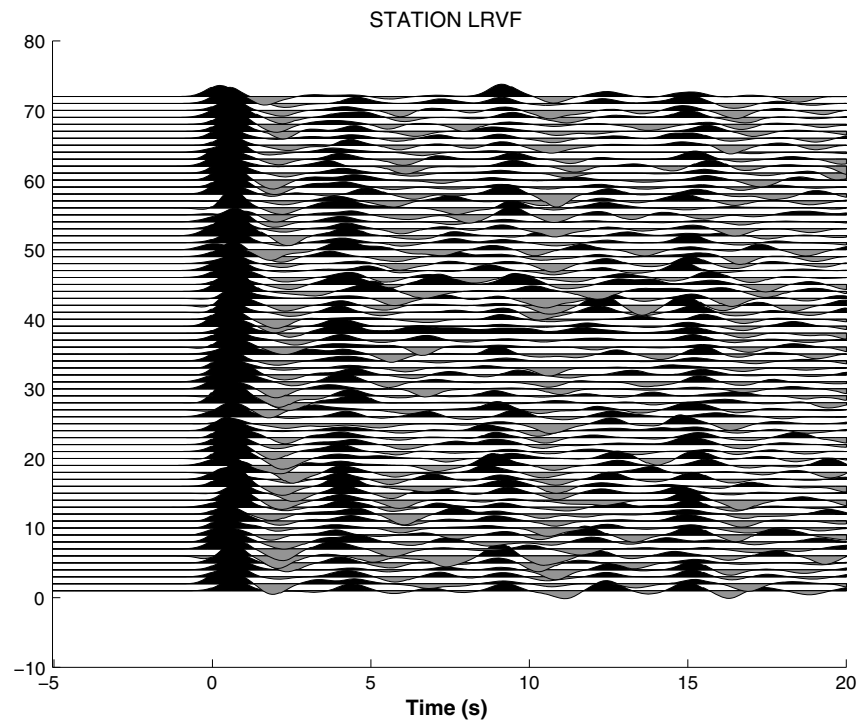
Figure 5. Receiver functions for permanent station LRVF (latitude 44.947^\circ , longitude -0.312^\circ ).
