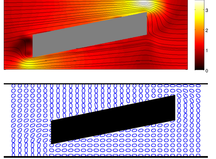
FIG. 2. (Color online) Maps of the velocity normalized by the average inlet velocity (top) and of the deformation quantified by the tensor \tilde{\sigma} (bottom), in the symmetric case a_c = a_d .
