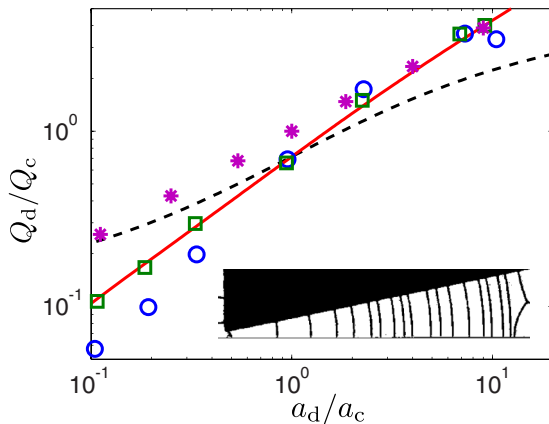
FIG. 4. (Color online) Flux ratio Q_d/Q_c plotted versus a_d/a_c . The experimental data for two different bubble areas are 0.11 \pm 0.02 cm 2 ( \square ) and 0.45 \pm 0.10 cm 2 ( \circ ). The dashed curve is from Eq. (5) with \mathcal{L}_c^*/\mathcal{L}_d^* = 0.80 . The solid curve is from Eq. (7) with \mathcal{L}_c^*/\mathcal{L}_d^* = 0.80 and B = 8.7 . The asterisks denote results from 3D simulations of a Stokes flow (Newtonian fluid, vanishing Reynolds number). The inset shows a zoom at the entrance of the divergent channel when it is narrow and the bubbles are big, showing the structure as a bamboo foam.
