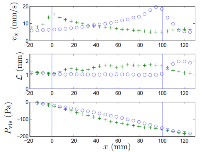
FIG. 3. (Color online) Shown, from top to bottom, are the velocity component v_x , length \mathcal{L} , and pressure (set to zero at x = -19 mm) as functions of x along the convergent [ \circ ; dash-dotted line in Fig. 1(b)] and divergent [ + ; dotted line in Fig. 1(b)] channels. The origin of the x axis is taken at the entrance of the two channels. Vertical lines indicate the locations of the entrance and exit of the two channels.
