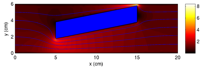
FIG. 5. (Color online) Map of the normalized local fluxes \|\mathbf{q}(x,y)\|/\langle q \rangle for the geometry such that a_2 = 9a_1 , with the obstacle and a few streamlines drawn in blue.
