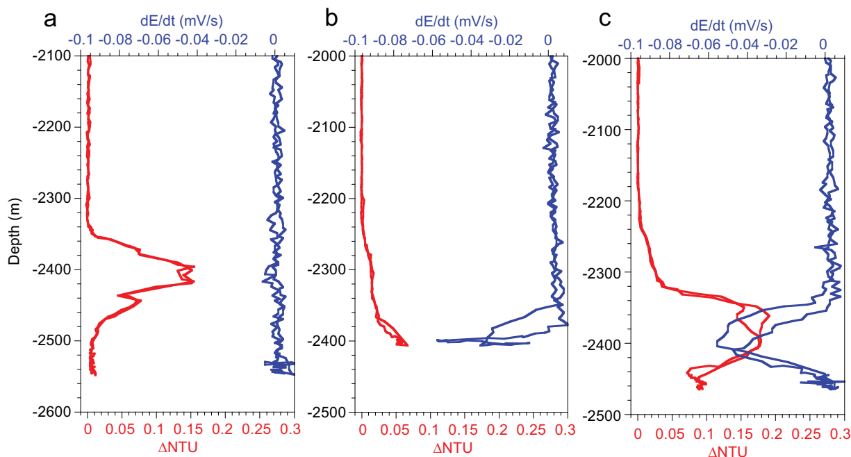
Figure 3. Typical MAPR profiles showing light backscatter anomaly as \Delta NTU (red) and oxidation-reduction potential as the time derivative of the ORP value (dE/dt (mV/s); blue). Vertical and horizontal scales identical for each plot. (a) A plume with high \Delta NTU but very weak dE/dt indicates an obvious plume from a source > \sim 1 km distant. (b) Near-bottom plume with both \Delta NTU and dE/dt anomalies implies a nearby source with a low buoyancy flux. (c) An above bottom plume with both \Delta NTU and dE/dt imply a nearby source with a higher buoyancy flux.
