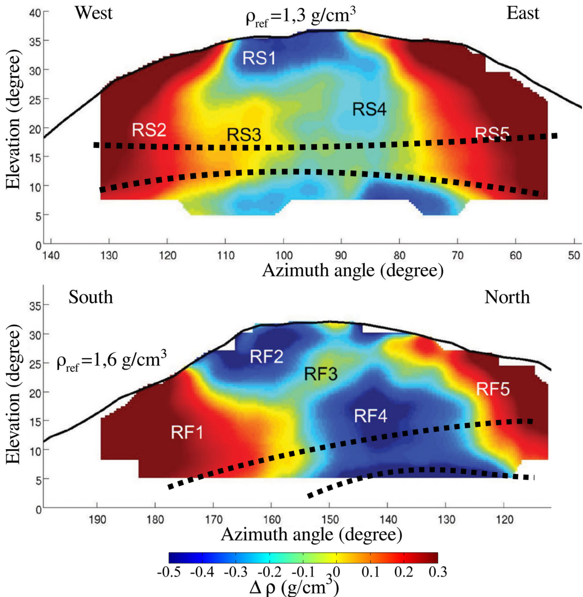
Figure 3. Density radiographies obtained with cosmic muon telescopes placed at the ‘Ravine Sud’ (top) and ‘Roche Fendue’ (bottom) locations (Leparre et al. 2012). Locations and angular ranges spanned by the radiographies are shown in Fig. 2: the ‘Ravine Sud’ radiography is roughly west–east oriented, and the ‘Roche Fendue’ is oriented south–north. The regions of the radiographies contained between the dotted lines correspond to radiography rays (see the Appendix for details) passing through the SERT cross-section limited by the electrode ring in Fig. 5.
