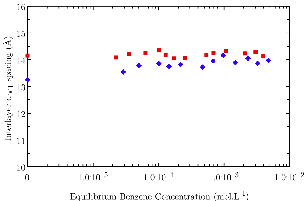
Figure 8: Evolution of the d_{001} basal spacing determined by the 00l reflection of the silicates sheets obtained from X-ray diffraction patterns of BDTA-Mt cationic organoclay (red squares) and C 10 E 3 -Mt nonionic organoclay (blue diamonds) after being impregnated in benzene solutions as a function of the equilibrium nonpolar hydrophobic compound concentration.
