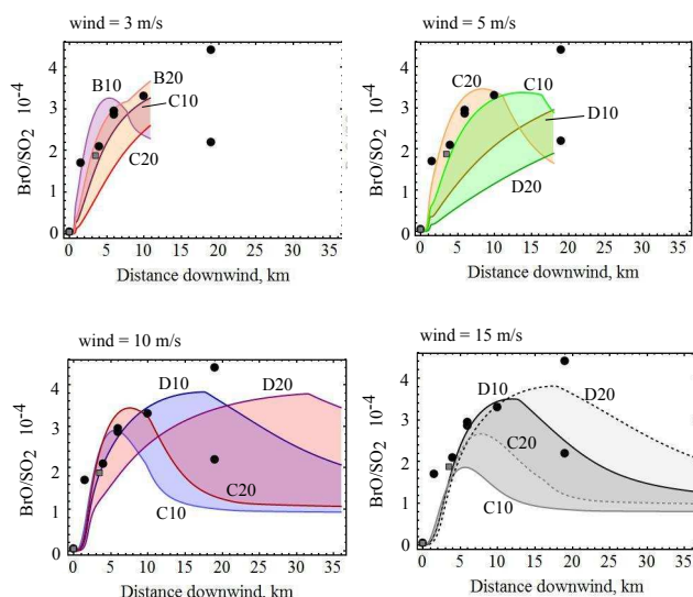
Figure 6. Simulated BrO/SO 2 over 1 h for the medium bromine emission, predicted for two emission flux scenarios (10 or 20 kg s -1 ), and for a range of wind speeds (3, 5, 10, 15 m s -1 ), and Pasquill–Gifford dispersion schemes (B, C, D). See text for details of the combinations. Model runs are compared to observations from Bobrowski et al. (2007) and Oppenheimer et al. (2006), shown as black circles and grey squares, respectively.
