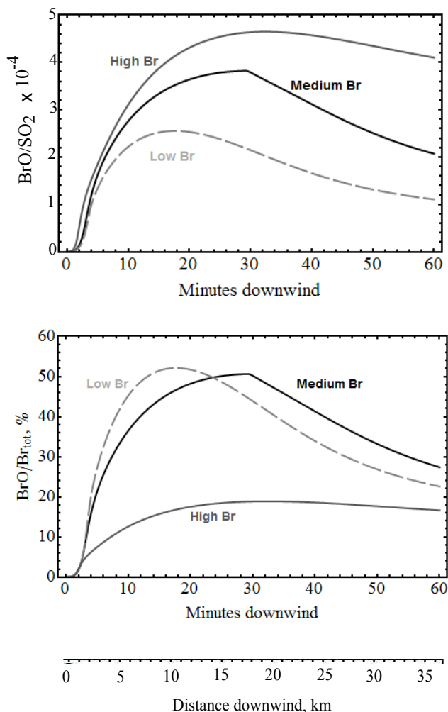
Figure 4. Predicted evolution in BrO/SO 2 (top) and BrO/Br tot ratios (bottom) over 1 h for the three different bromine emission scenarios. Model runs correspond to those shown in Fig. 3 assuming V_A : V_M = 5 : 95 for the high-temperature initialisation.
