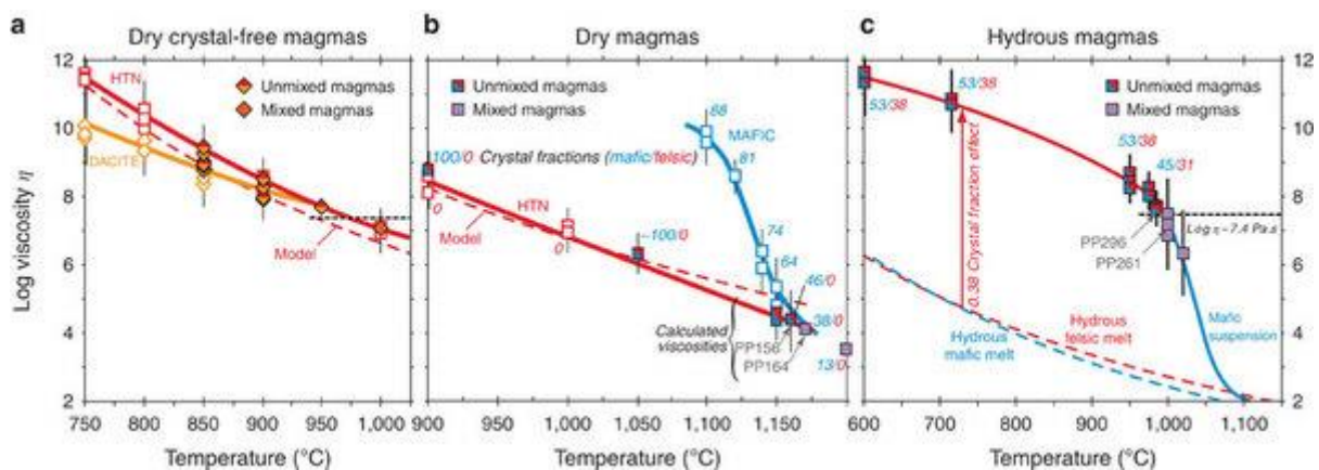
Figure 2: Experimental magma viscosities during mixing.
