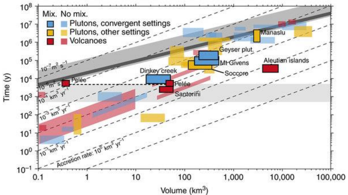
Figure 9: Relationships between volumes of reservoir and cooling times.
