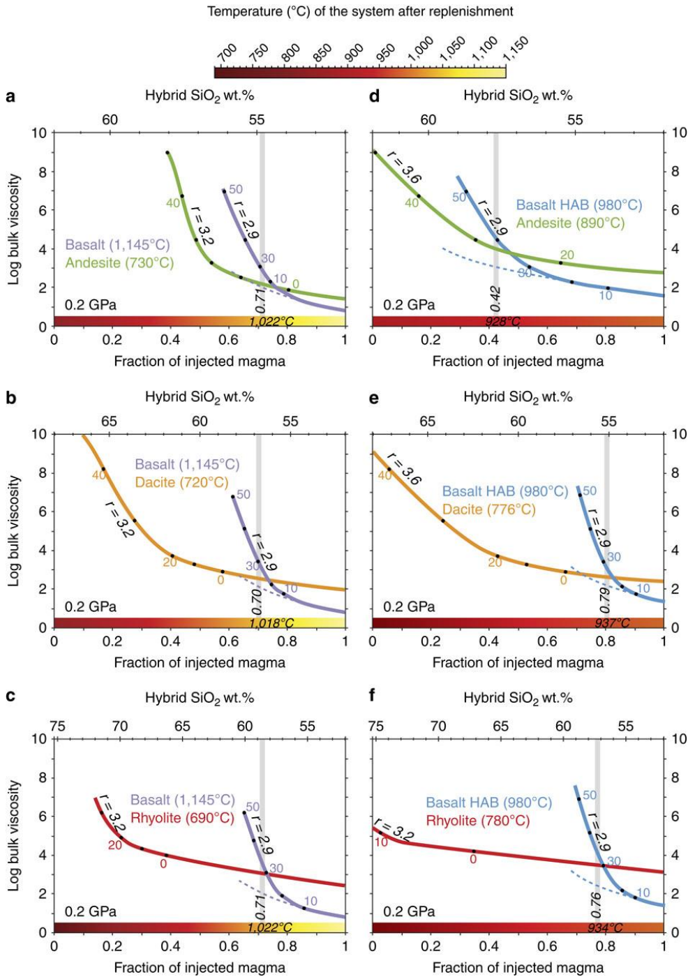
Figure 6: Evolution of felsic and mafic magma viscosities with fraction of mafic magma.
