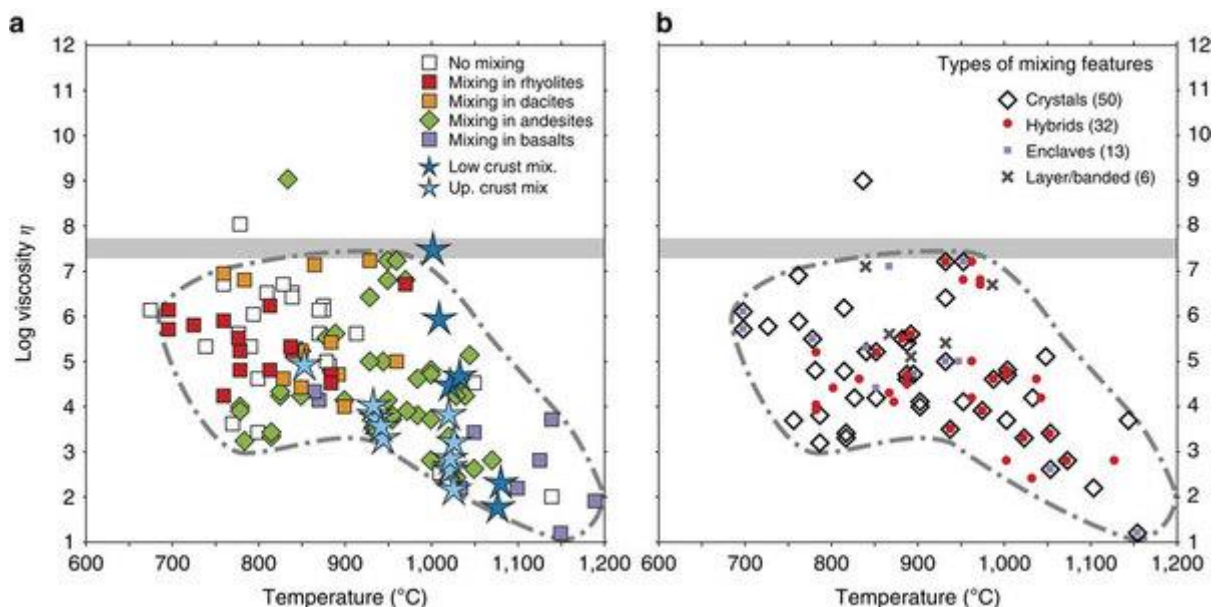
Figure 8: Viscosities of natural magmas.
