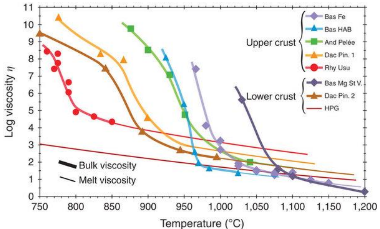
Figure 4: Evolution of magma viscosity with temperature.
