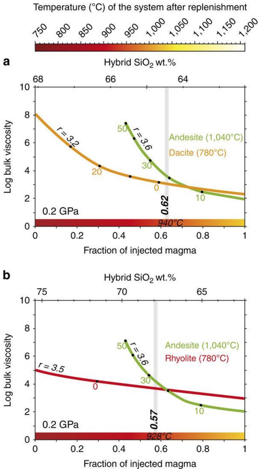
Figure 7: Evolution of felsic and intermediate magma viscosities with fraction of intermediate magma.
