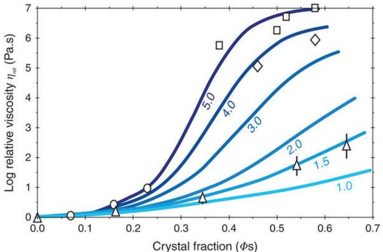
Figure 3: Evolution of magma viscosity with crystal fraction and shape ratio.
