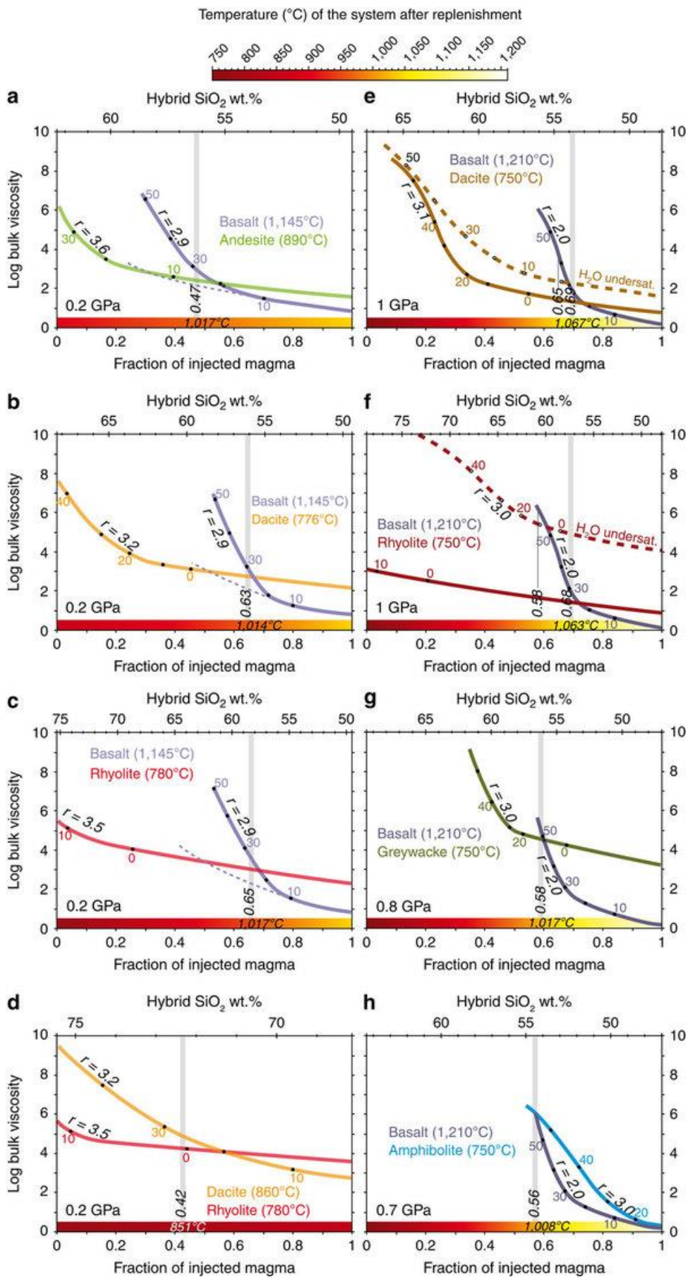
Figure 5: Evolution of felsic and mafic magma viscosities with fraction of mafic magma.
