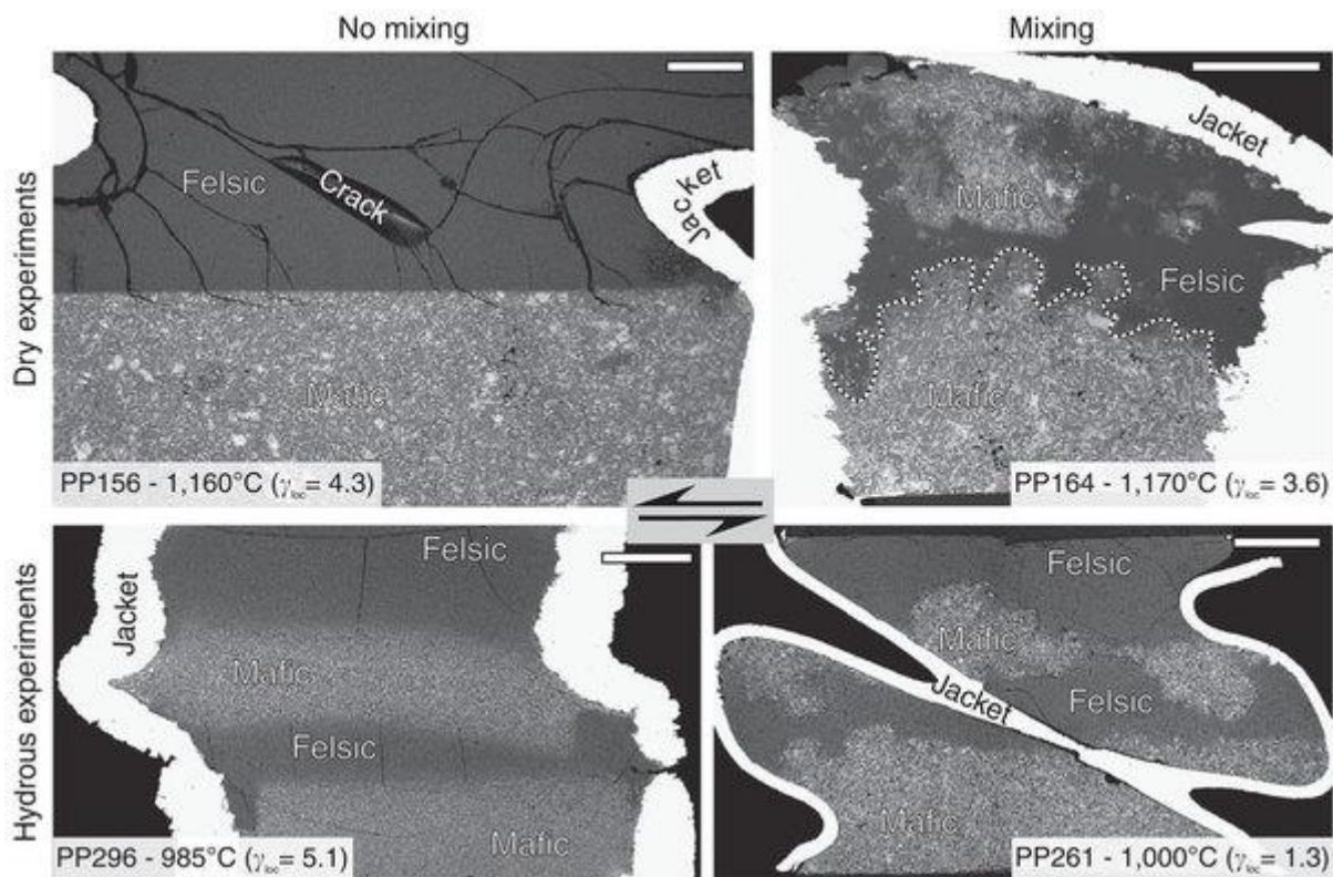
Figure 1: Illustration of experimental textures.
