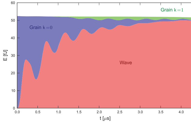
Figure 8: Evolution of the distribution of energy in the system containing two glass grains fixed by springs and surrounded by water
