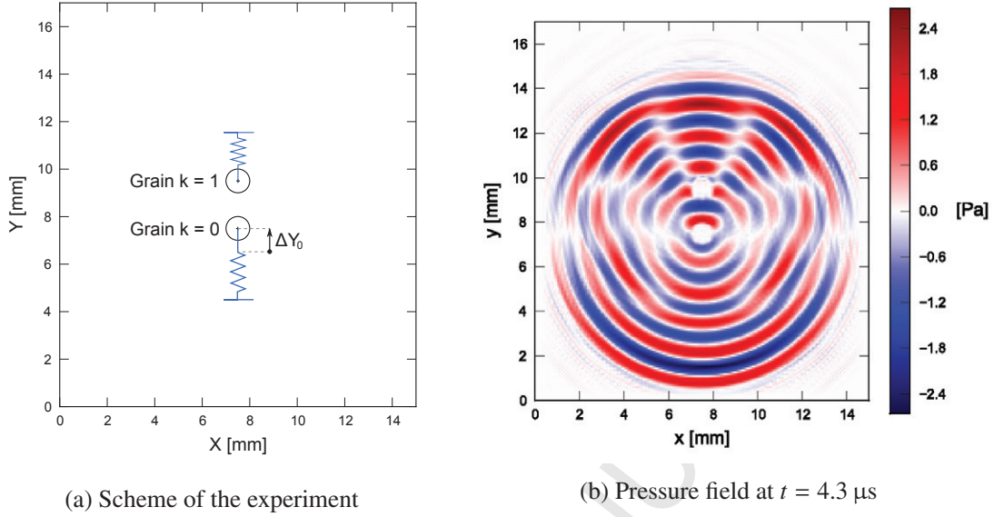
Figure 7: Numerical experiment of two movable grains fixed by springs. Fig. 7a shows a simplified representation of the experiment and Fig. 7b the pressure field at the final time t = 4.3 \mu\text{s} .
