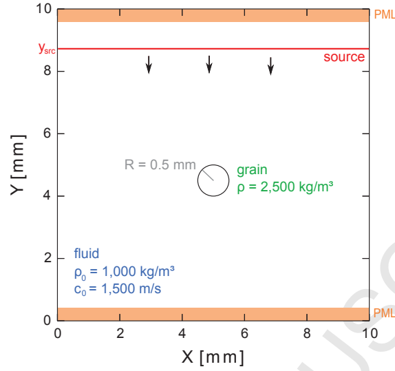
Figure 3: Scheme of the experiment with 1 grain
