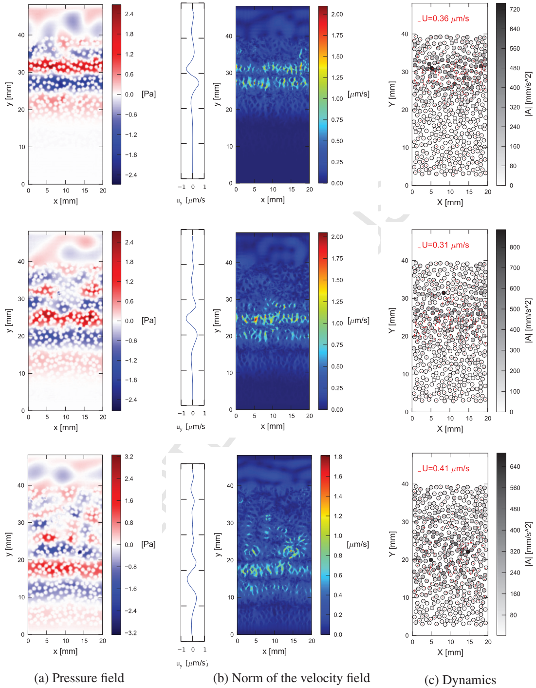
Figure 10: Propagation of a pulse through a granular suspension at t = \{25; 30; 35\} \mu\text{s} .
