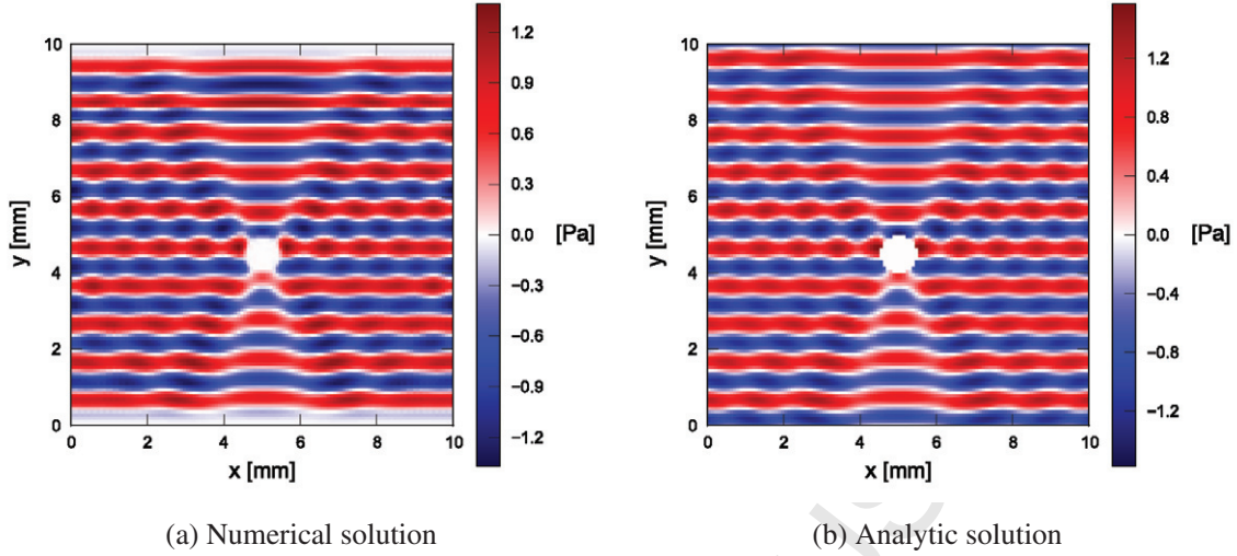
Figure 4: Numerical solution of the total pressure field computed using the fictitious domain method (4a) versus the analytic solution (4b) for h_\Omega = 1/12 mm.
