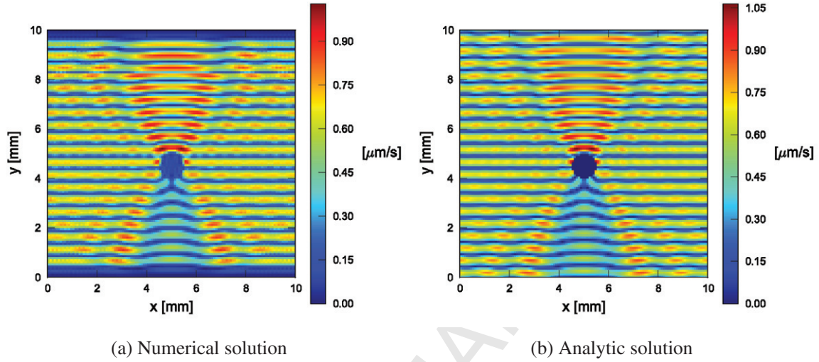
Figure 5: Numerical solution of the norm of the total velocity field computed using the fictitious domain method (5a) versus the analytic solution (5b) for h_{\Omega} = 1/12 mm.
