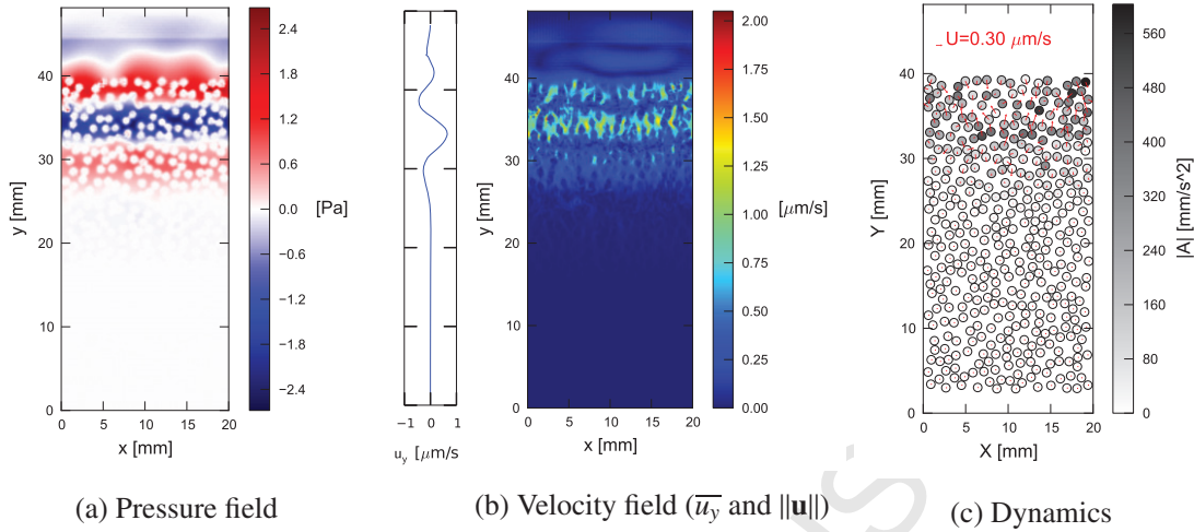
Figure 9: Propagation of a pulse through a granular suspension at t = 20 \mu\text{s} . Fig. (a) shows the acoustic pressure field, Fig. (b) the mean of the y-component and the norm of the velocity field and Fig. (c) positions, velocities (represented by red arrows) and acceleration (in grayscale) of each grain.
