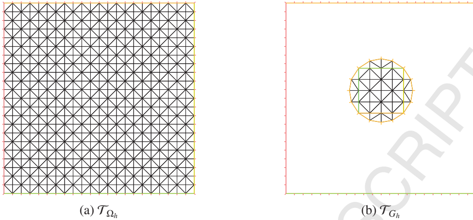
Figure 2: The regular grid \mathcal{T}_{\Omega_h} (on the left) is the grid where the physical variables \mathbf{u} and p are computed and the unstructured grid \mathcal{T}_{G_h} (on the right) is the domain of the Lagrange multipliers.
