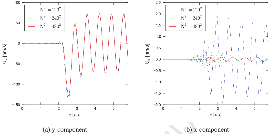
Figure 6: Velocity of the grain function of the time computed using the fictitious domain method for several discretizations.
