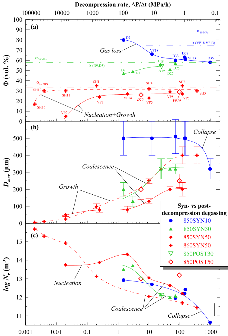
Fig. 3. Time evolution of the syn-decompression degassing (filled symbols; time is decompression duration) and post-decompression degassing (outlined symbols; time is time spent at P_f ) showing (a) \Phi , (b) D_{\text{max}} , and (c) N_v , for 850SYN50, 850SYN30, 850SYN10, and 860SYN50; The maximum error of the measurements is given by the black vertical lines on the right-hand side of the diagrams, except in (b). In (a), labels refer to the run numbers as in Table 1 and the dash-dot lines show \alpha as given in Table 2; in (c), only the samples with crystal content \psi \leq 16 vol% are shown (see text for justification); 860SYN50 data from Martel and Schmidt (2003). (For interpretation of the references to color in this figure legend, the reader is referred to the web version of this article.)
