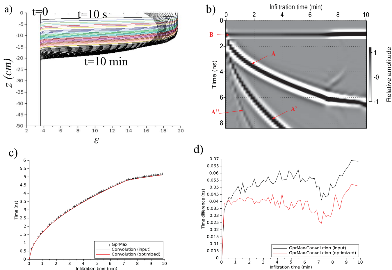
Figure 4. Numerical example of a falling head infiltration: (a) permittivity profiles (curves are plotted every 10 s), (b) radargram simulated with GprMax 2D (reflection A is coming from the wetting front, B is the direct wave, A' and A'' are multiples of reflection A ), (c) comparison between TWT obtained by: crosses, picking reflection A peaks on radargram (Figure 4b), black line, using the convolution algorithm with p_{in} , red line, using the convolution algorithm with p_{op} . (d) Differences between the TWT using: black line, the convolution algorithm with p_{in} and the radargram (Figure 4b), red line, the convolution algorithm with p_{op} and the radargram (Figure 4b).
