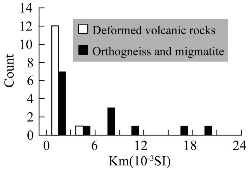
Figure 6. Distribution of the bulk magnetic susceptibility of magmatic rocks in the Changle-Nan'ao Belt.
