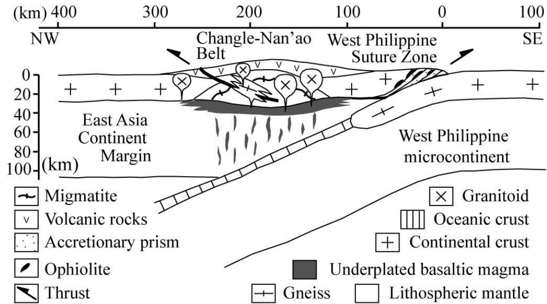
Figure 12. Interpretative lithosphere-scale cross section of the East Asia Continental Margin during the Early Cretaceous. The Changle-Nan'ao Belt is interpreted as a magmatic arc back-thrusted to the NW in response to the continental subduction, and collision of the West Philippines microcontinent below the South China Block.
