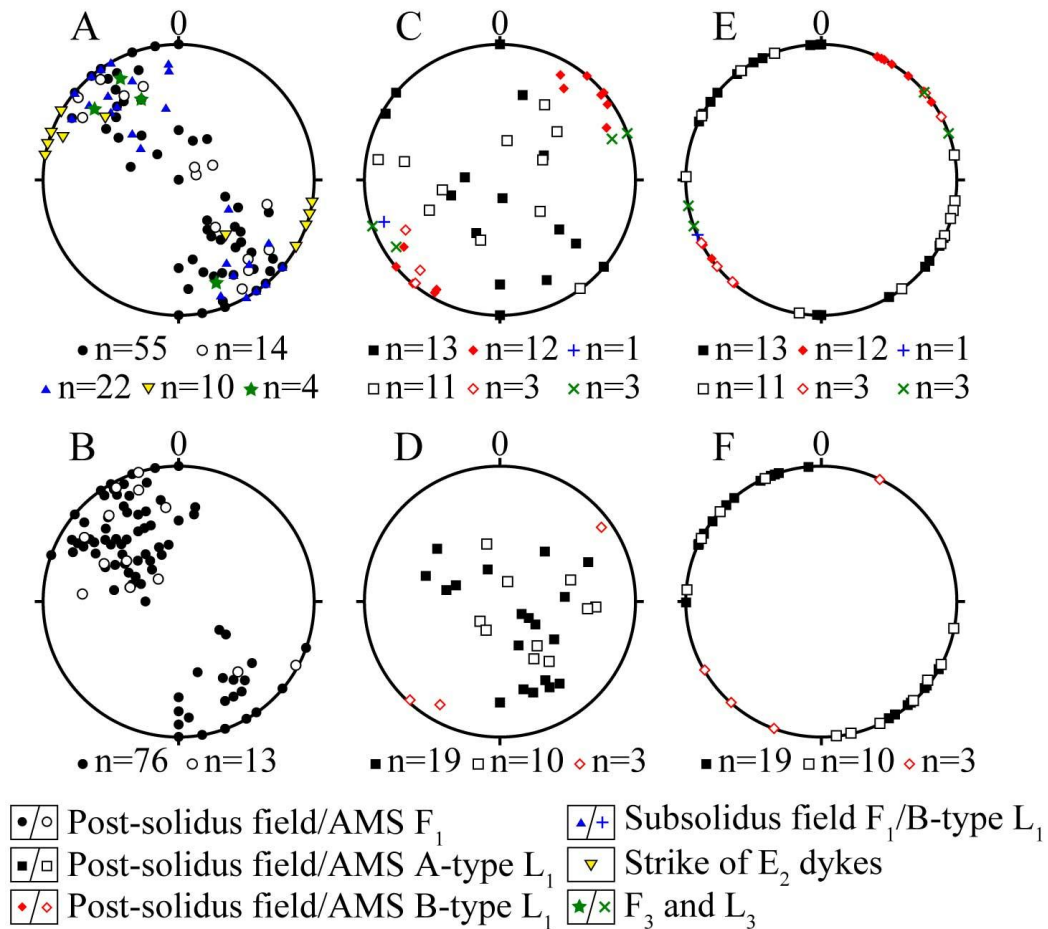
Figure 5. Equal-area lower hemisphere projections of total fabrics of the Changle-Nan'ao Belt. A: foliation pole of gneiss, syn-tectonic granitoid, E_3 shear zone, and strike of E_2 dykes; B: foliation pole of deformed volcanic rocks; C: lineation of E_1 gneiss, E_1 sub-solidus granitoid and E_3 narrow shear zone; D: lineation of deformed volcanic rocks; E: lineation of gneiss, E_1 sub-solidus granitoid and E_3 shear zone after correcting foliation to flat; F: lineation of deformed volcanic rocks after correcting foliation to flat. Solid and open circles/rectangles represent E_1 field and AMS foliation/A-type lineation. Solid and open diamonds represent E_1 field and AMS B-type lineation, Triangle and cross represent sub-solidus field foliation and B-type lineation, reverse triangle represents strike of E_2 dykes, Star and oblique cross represent E_3 foliation and lineation, respectively. The stereo projection of the AMS ellipsoid, please refer to Appendix 3.
