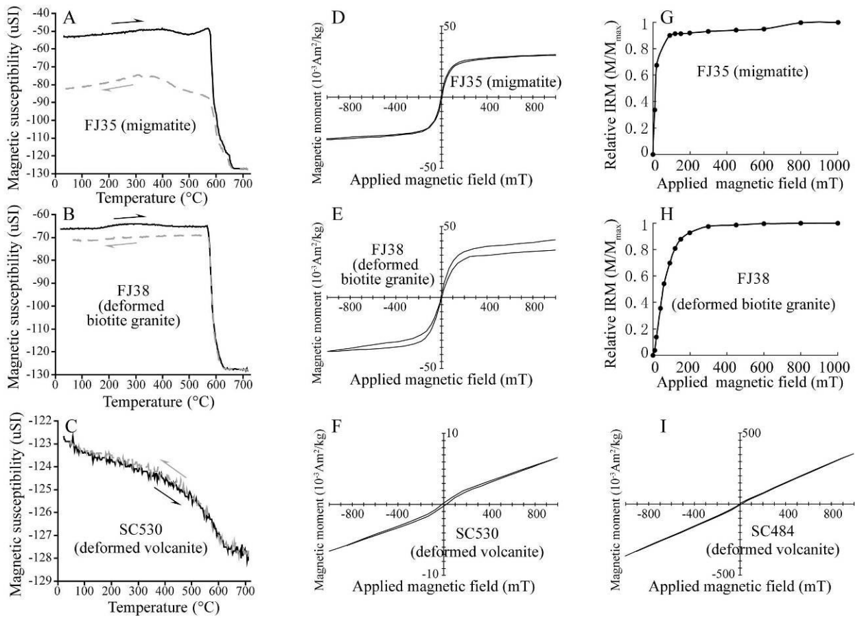
Figure 7, Thermal-Susceptibility, Isothermal Remanent Magnetization (IRM), Hysteresis Loop diagram of the deformed rocks of the Changle-Nan'ao Belt. The analyzed samples are located in Table 1.
