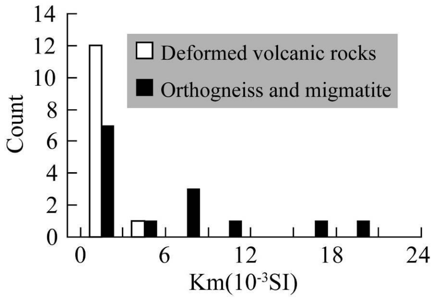
Figure 6. Distribution of the bulk magnetic susceptibility of magmatic rocks in the Changle-Nan'ao Belt.
