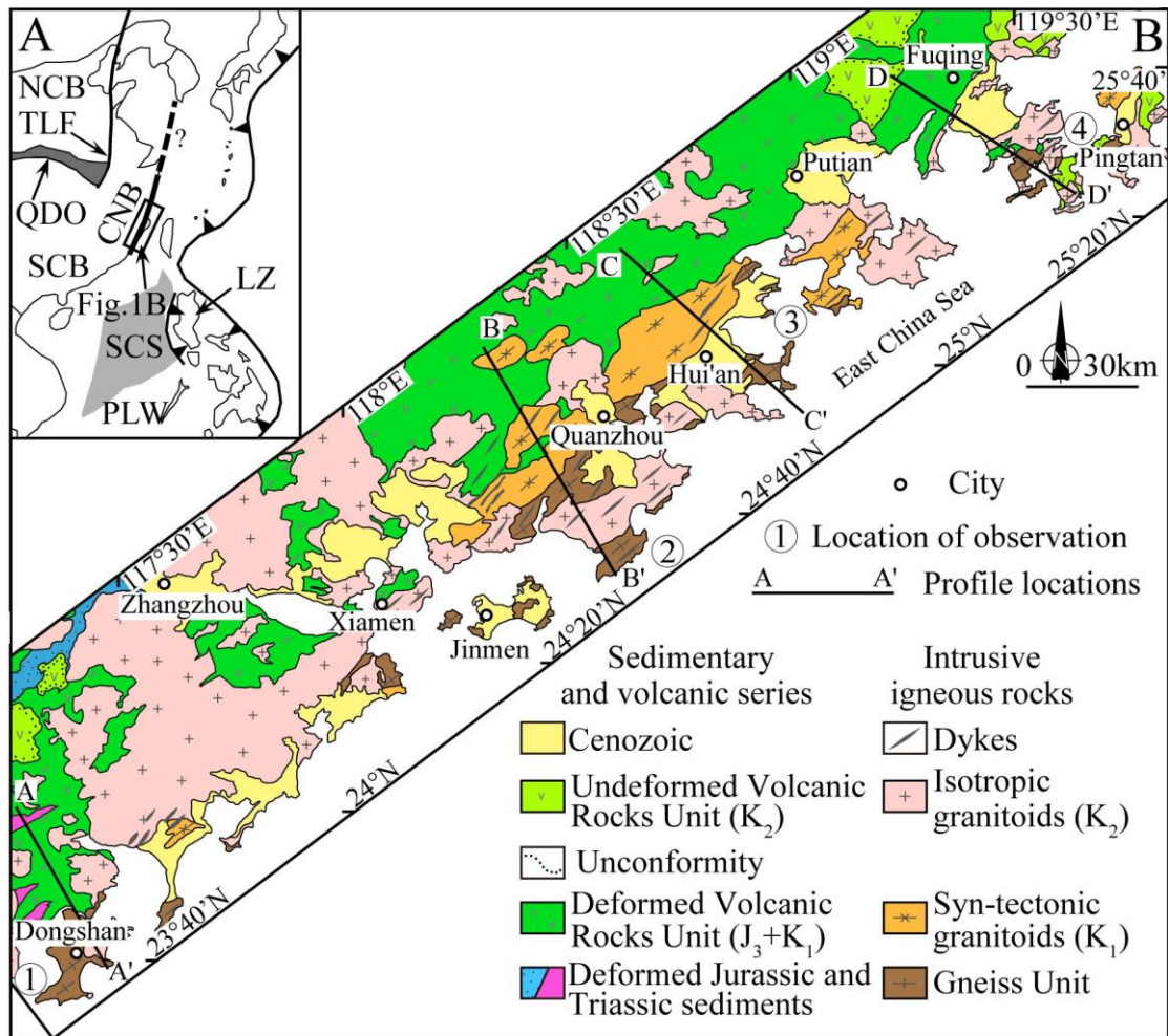
Figure 1. A: Sketch map of the present East Asia Continental Margin geodynamics. NCB: North China Block; TLF: Tan-Lu fault; QDO: Qinling-Dabie Orogen; SCB: South China Block; CNB: Changle-Nan'ao Belt; SCS: South China Sea; LZ: Luzon Island; PLW: Palawan Island. B: Sketch geologic map of the Changle-Nan'ao Belt.
