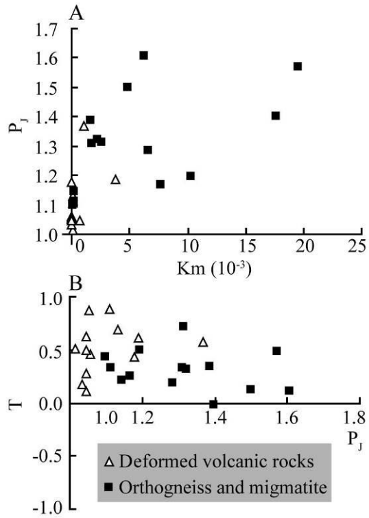
Figure 9. AMS scalar parameters for each site and main lithologies. A: P_J (corrected anisotropy degree) vs. Km (mean bulk magnetic susceptibility in 10^{-3} SI); B: T (shape parameter) vs. P_J (corrected anisotropy degree). The calculations of T and P_J can be found in Jelinek (1981).
