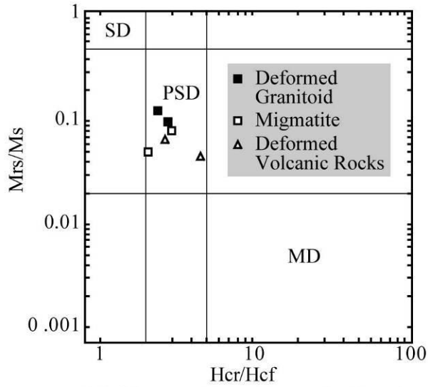
Mrs/Ms versus Hcr/Hc for samples from the Changle-Nan'ao Belt, with the boundaries of SD and MD behaviours for magnetite taken from the values of Dunlop (2002)
