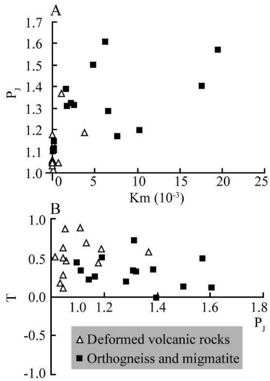
Figure 9. AMS scalar parameters for each site and main lithologies. A: P_J (corrected anisotropy degree) vs. K_m (mean bulk magnetic susceptibility in 10^{-3} SI); B: T (shape parameter) vs. P_J (corrected anisotropy degree). The calculations of T and P_J can be found in Jelinek (1981).
