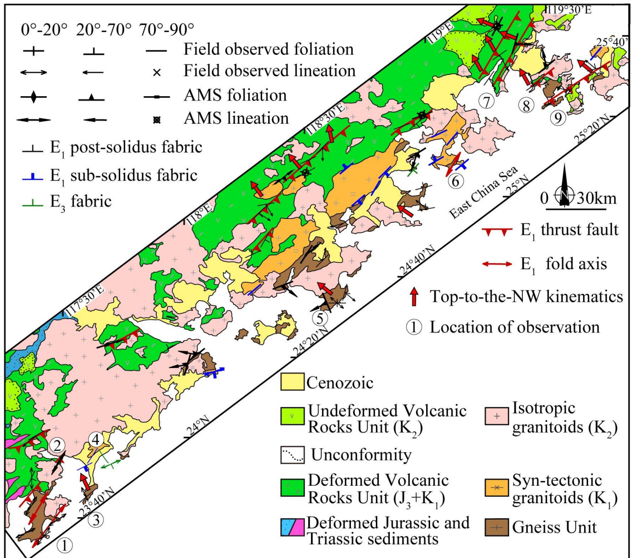
Figure 3. Representative field observed fabric and laboratory measured magnetic fabric of CNB and their structural interpretation. The dip of the foliation/magnetic foliation and the plunge of the lineation/magnetic lineation, please refer to Appendix 2.
