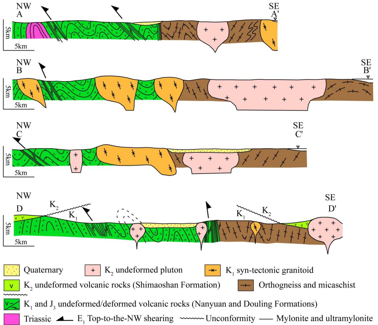
Figure 4. NW-SE representative cross sections illustrating the bulk architecture of the Changle-Nan'ao Belt. Profile locations refer to line AA', BB', CC' and DD' in Fig. 1B.
