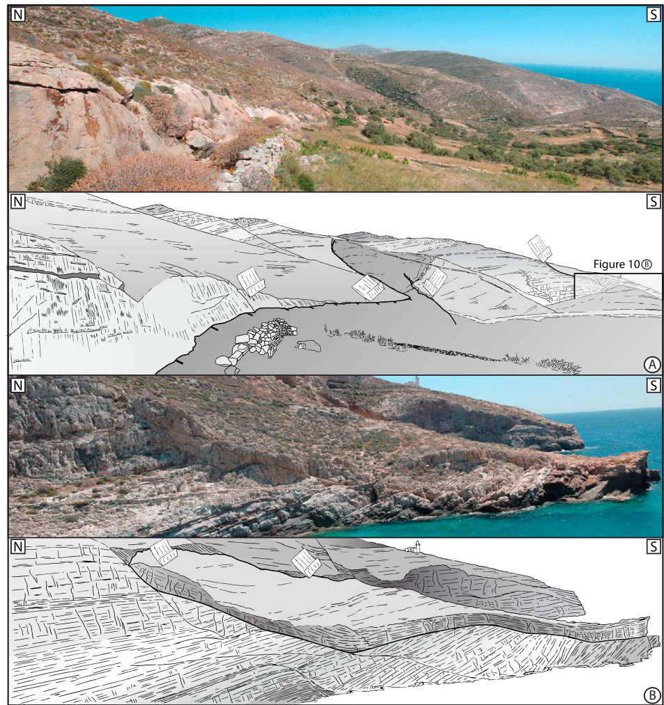
Figure 10. Mesoscale brittle structures. (a) Large-scale listric normal faults. (b) Flat-ramp-flat extensional system located approximately 1 km south of Figure 10a. Both outcrops show hanging wall displacements toward the south (Figure 4). Kinematics of mesoscale structures is consistent with the microscale brittle structures. See Figure 4 for location.
