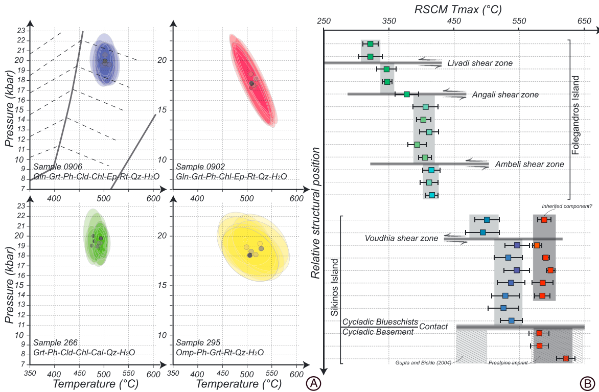
Figure 12. P-T constraints. (a) Average P-T results presented for the four samples. For the sake of clarity, P-T points and related error bars are shown only for the runs performed for H 2 O activity = 1. Error brackets are based on the 1 s uncertainties on pressure and temperature results. (b) RSCM peak temperature results versus structural relative position in the metamorphic succession. Indicated is the position of the main shear zones deduced from the structural approach. Error brackets correspond to intrasample heterogeneity.
