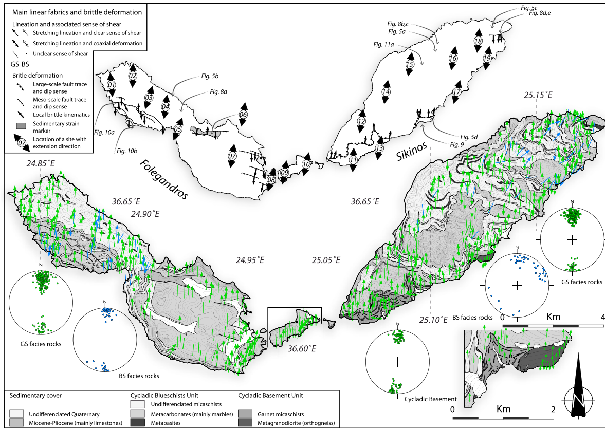
Figure 4. Stretching lineations of Sikinos and Folegandros islands. Geological and stretching lineation map of Sikinos and Folegandros Islands. Stretching lineations in both the Cycladic Blueschists and the Cycladic Basement units are presented in Schmidt's lower hemisphere equal-area projection. Lineations associated to blueschist-facies rocks are indicated in blue; lineations associated to greenschist-facies rocks in green either on the map or on the projections. Detailed map of the northern tectonic window of the Cycladic Basement unit surrounded by the Cycladic Blueschists unit. Note that the orientation of the stretching lineation remains constant across the Cycladic Blueschists/Cycladic Basement contact. In addition, both top-to-the-north and top-to-the-south senses of shear are present in the Cycladic Basement unit (see text for details). Simplified geological map showing the results of the fault slip data inversion together with traces of main brittle structures and their local kinematics. Also indicated is the position of the pictures of Figures 5 and 8–11.
