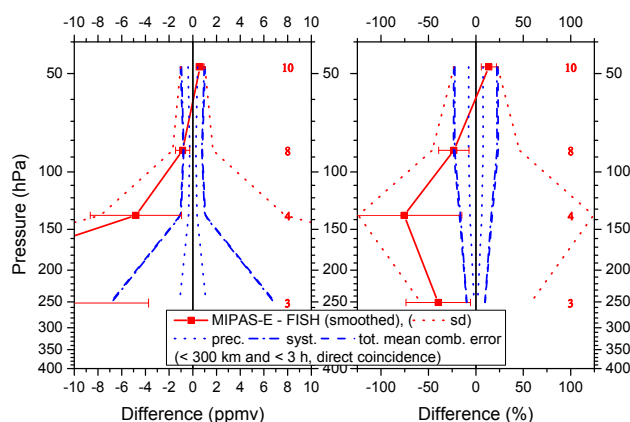
Fig. 8. Absolute (left) and relative (right) H 2 O differences (red squared lines) between MIPAS-E and the stratospheric hygrometer FISH for all Geophysica flights carried out above Italy and northern Sweden within a direct coincidence limit of 300 km and 3 h together with mean combined precision (blue dotted lines), systematic (blue dash-dotted lines), and total errors (blue dashed lines) as well as standard deviation (red dotted lines) and the standard error of the mean, plotted as error bars. FISH profiles were smoothed with the averaging kernel of MIPAS-E. Red values (along the right-hand y-axes) indicate the number of collocations at corresponding pressure levels.
